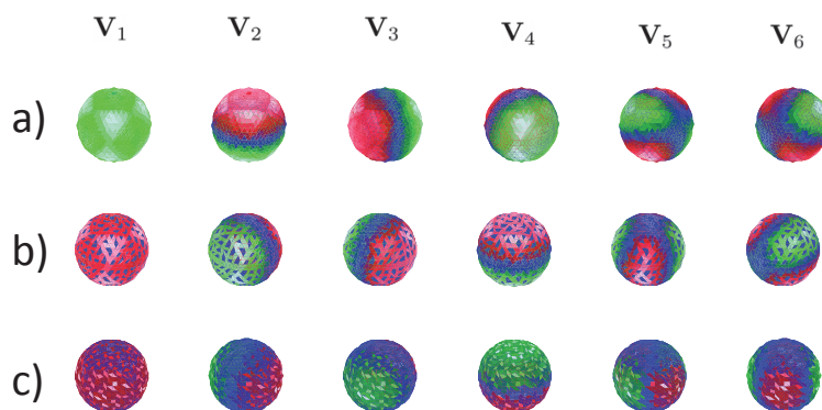
Fig. 8. Plot of the first columns of [\mathbf{U}] from the SVD of [\mathcal{S}_{(\Gamma_0, \Gamma)}] at f = 100 Hz. a) linear elements, b) quadratic elements, and c) cubic elements.
