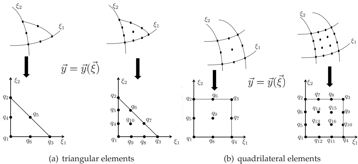
Fig. 2. Boundary elements used for iso-parametric transformation: linear, quadratic and cubic elements.
