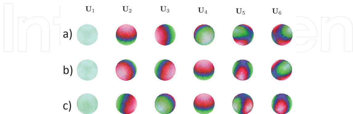
Fig. 7. Plot of the first columns of [\mathbf{U}] from the SVD of [\mathcal{S}_{(\Gamma_0, \Gamma)}] at f = 100 Hz. a) linear elements, b) quadratic elements, and c) cubic elements.
