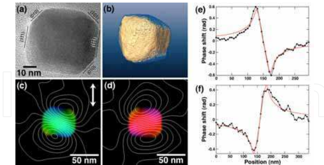
Fig. 7. (a) High-resolution TEM image of a 50-nm-diameter magnetite crystal from a magnetotactic bacterial cell (recorded by M. Pósfai). (b) Three-dimensional morphology of the same particle obtained using high-angle annular dark-field electron tomography (recorded by R.K.K. Chong). (c,d) Remanent magnetic states of the particle recorded at room temperature and at 90 K, respectively. The double arrow shows the applied field direction before reducing the experimental field to zero and recording holograms. (e,f) Data points in the line profiles show the magnetic contribution to the phase shift across the particle measured (e) at room temperature and (f) at 90 K. The red lines show least-squares fits to the data points, yielding values of B_{\perp}=0.60(\pm 0.12) T at room temperature and B_{\perp}=0.46(\pm 0.09) T at 90 K.
