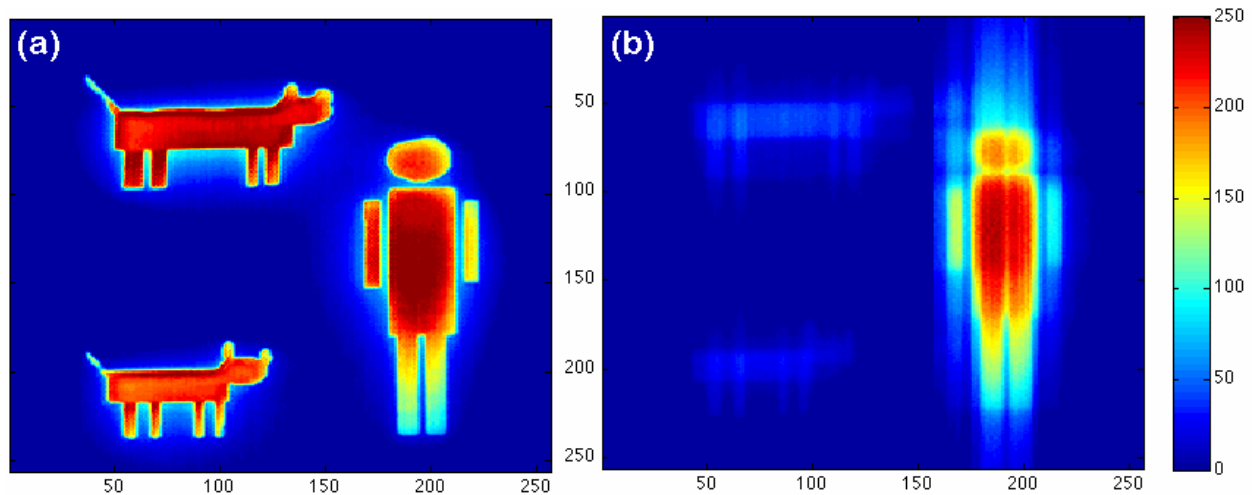
Fig. 20. Resulting intensity images generated from the Fresnel lenses in the visible range of spectrum. (a) Resulting image from the conventional (quadratic phase profile) lens; (b) resulting image from the proposed lens (cubic phase profile). One can note the enhancement of the human body intensity distribution
