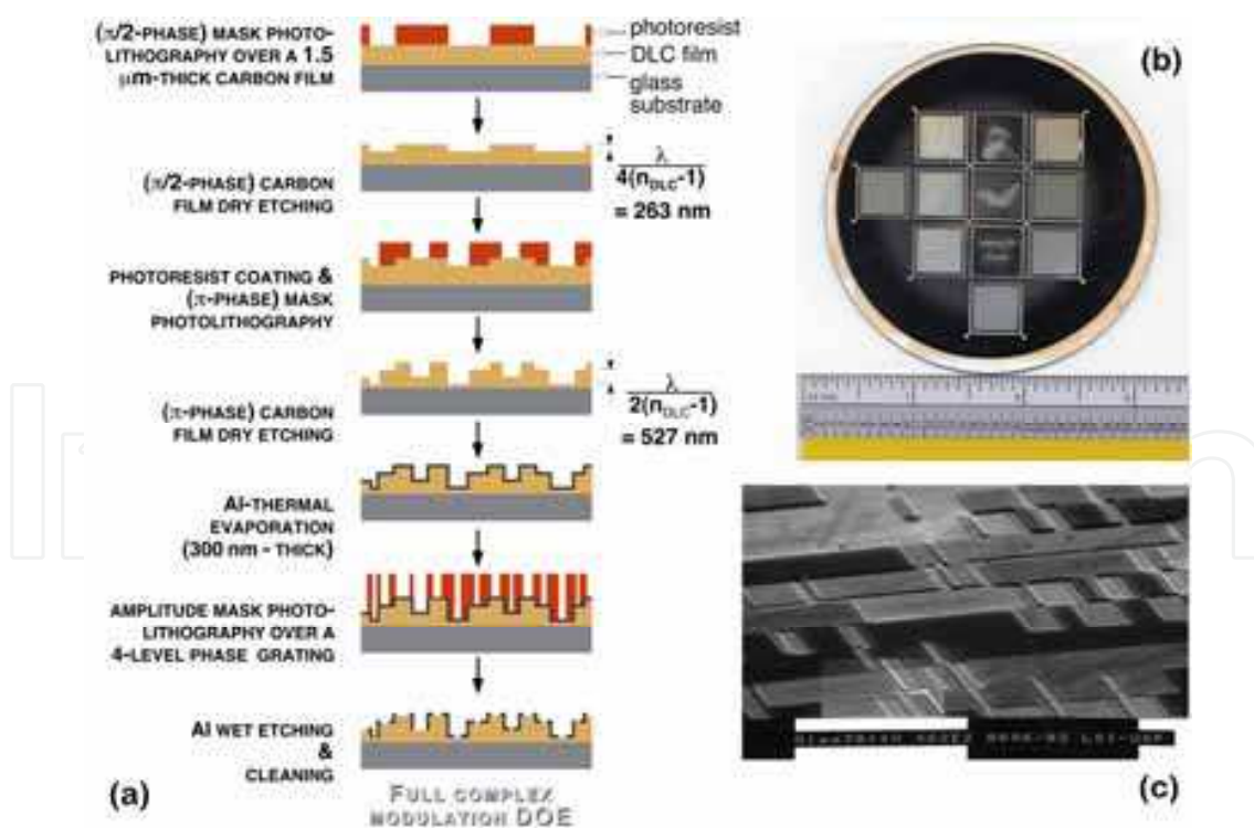
Fig. 14. (a) Schematic view of the fabrication of the full complex amplitude modulation CGH; (b) 3-inch diameter glass substrate, with 12 different CGHs fabricated. (c) Scanning electron microscope picture with details of the geometry of the rectangular pixels. Reprinted with permission of SPIE (Neto, L. G., 2004).
