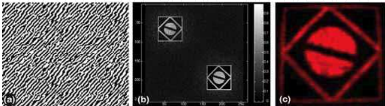
Fig. 4. (a) 64 \times 64 pixels binary amplitude-only modulation hologram; (b) numerical reconstruction, with a reconstruction plane of 256 \times 256 pixels; (c) Optical reconstruction. Only one image is shown; the DC central spot and the twin image were suppressed.
