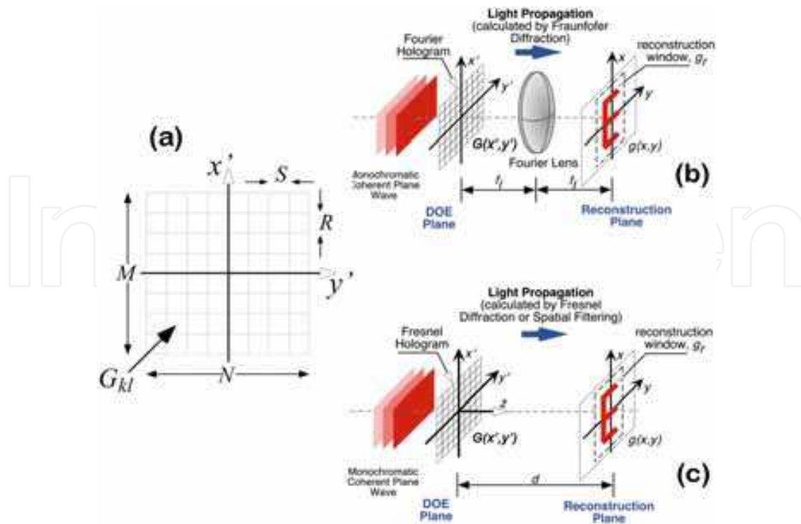
Fig. 1. (a) Hologram structure; (b) Optical reconstruction of Fourier-type CGH illuminated; (c) Reconstruction of a Fresnel-type CGH, obtained by the free space light propagation of g(x',y') along distance d . Reprinted with permission of SPIE (Neto, L.G. 2004).
