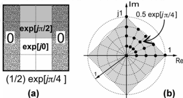
Fig. 8. (a) Structure of a particular cell with complex transmittance of amplitude equal to 0.5 and phase equal to \pi/4 ; (b) all the possible value (black dots) of amplitude and phase within the first quadrant, as well as, the particular value of the cell of figure (a). Reprinted with permission of OSA (Cirino, G. A., 2010).
