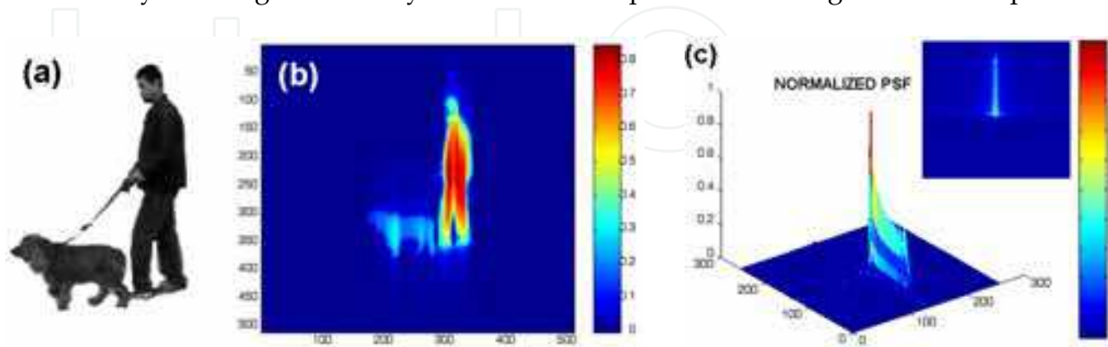
Fig. 18. Numerical simulation of the performance of the cubic phase mask to be embedded in the sensor's Fresnel lens array (a) Input test image used in the computer simulation; (b) corresponding simulated output image, normalized to its maximum value; (c) normalized PSF distribution of the optical system. One can note that the image of the human silhouette has higher brightness when compared to the image of a small pet.
