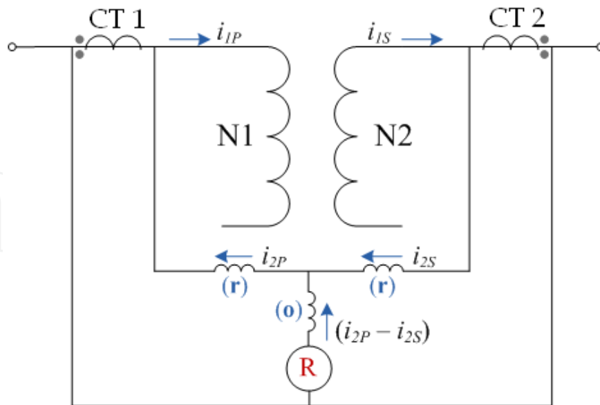
Fig. 3. Differential relay connections.
