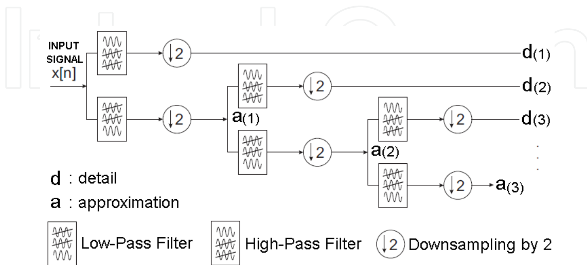
Fig. 2. DWT filter bank framework.
