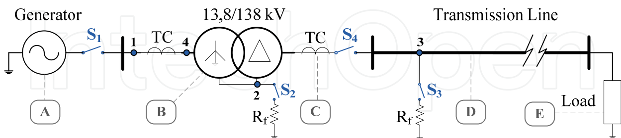
Fig. 6. Simulated electric power system.
