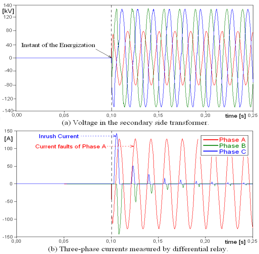
Fig. 8. Energization and internal faults simulation on PT.
