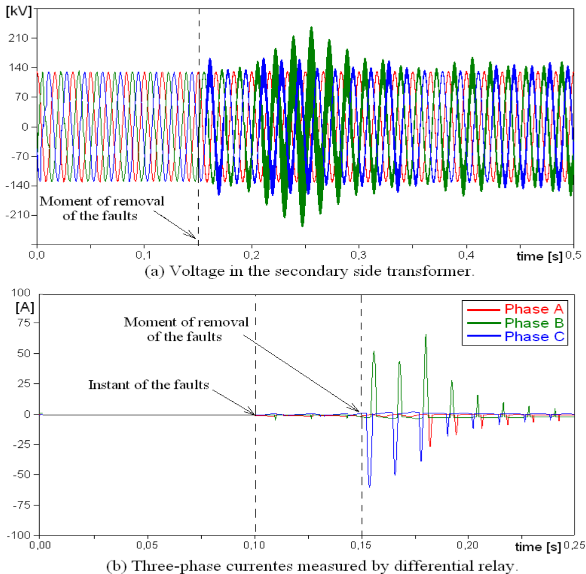
Fig. 9. External faults removal simulation.
