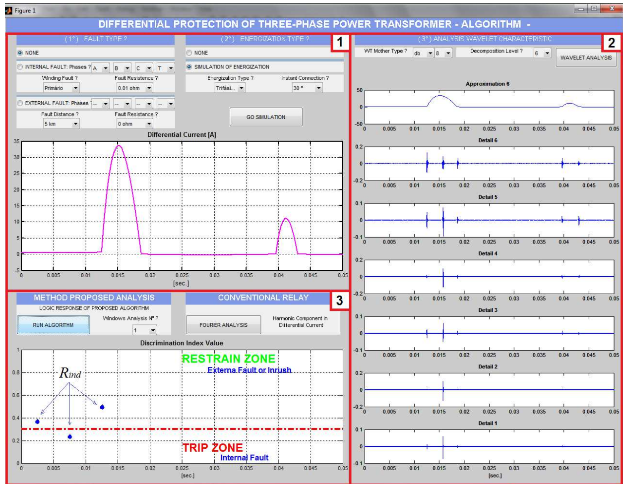
Fig. 5. Graphical implementation in MATLAB® environment.
