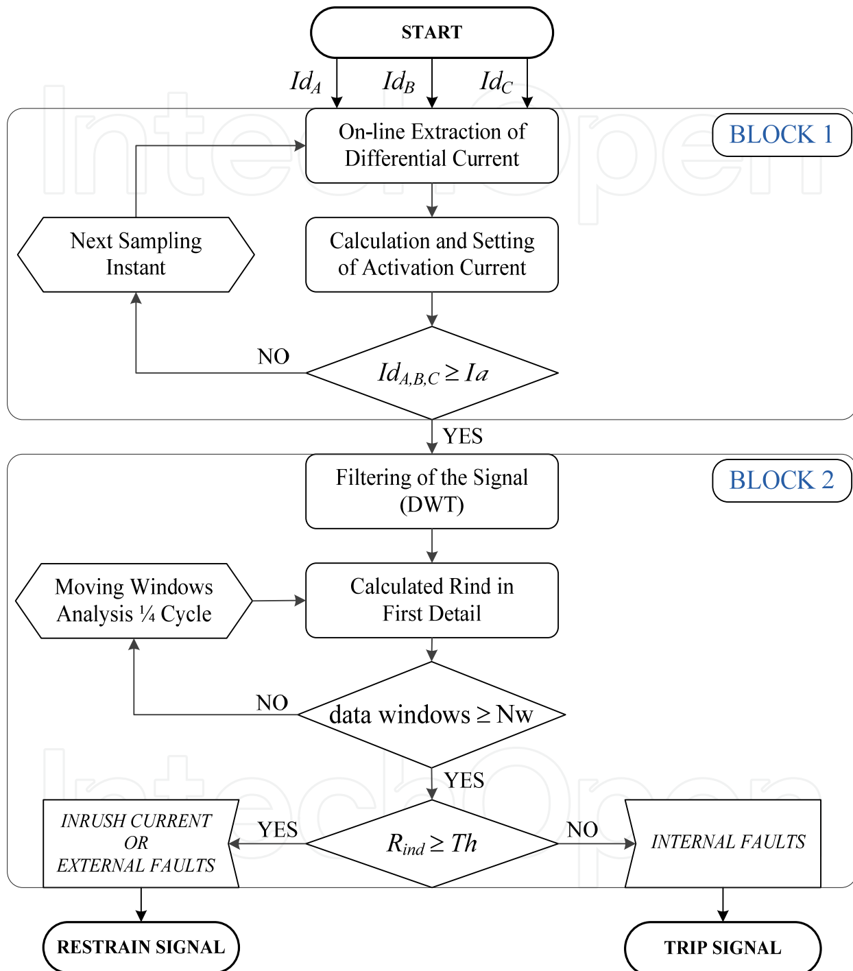
Fig. 4. Proposed Algorithm's Operation Scheme.
