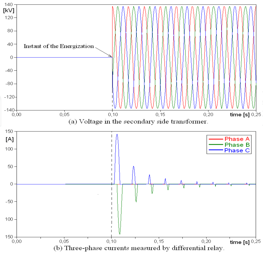
Fig. 7. Energization simulation on PT.
