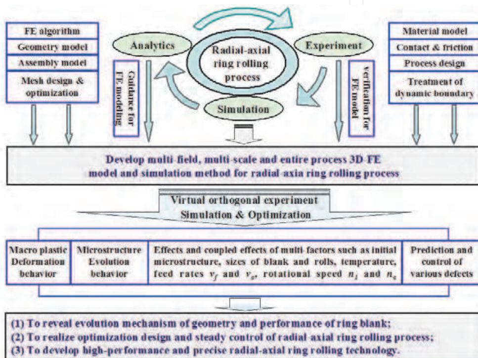
Fig. 3. High-end research route for radial-axial ring rolling technology
