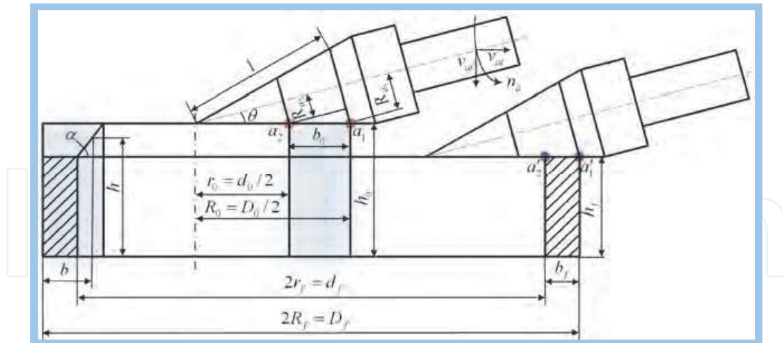
Fig. 7. Position variation of the upper conical roll before and after rolling
