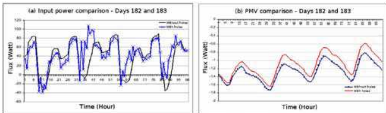
Fig. 15. Input power and PMV comparisons
