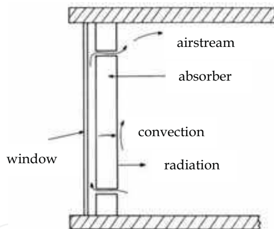
Fig. 12. Trombe-Michell recycling wall set-up (Sfeir, 1981)
