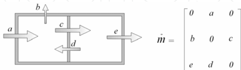
Fig. 3. Interzonal airflow rates matrix
