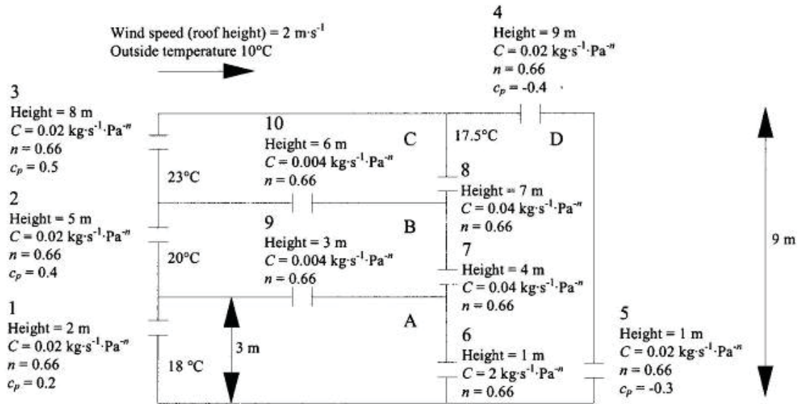
Fig. 6. TN 51 Test case
