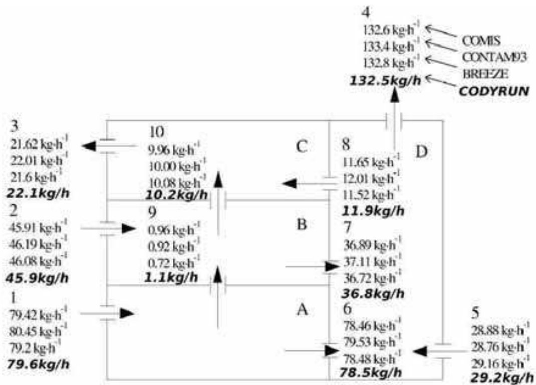
Fig. 7. Intermodel airflow comparison
