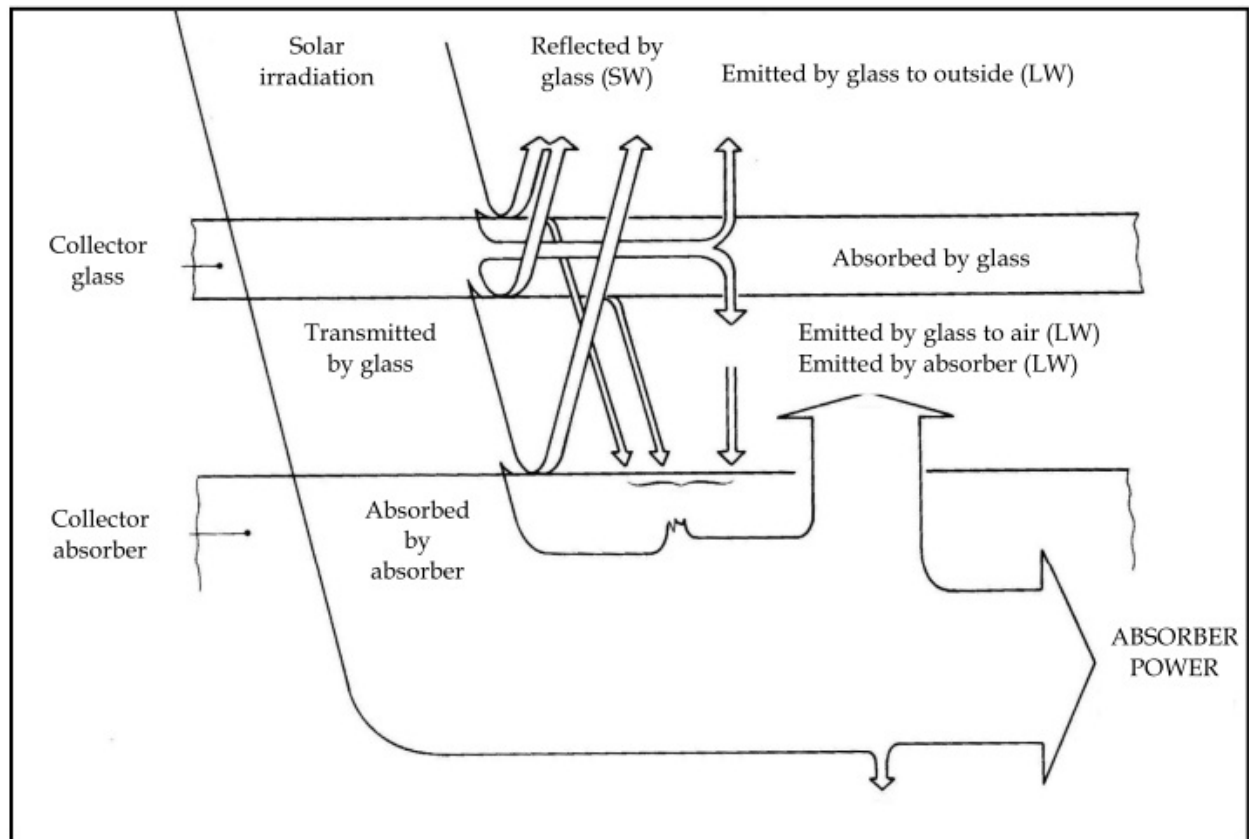
Fig. 9. Solar irradiation absorption process.
