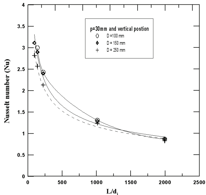
Fig. 13. Nusselt number versus L/d_i ratio.
