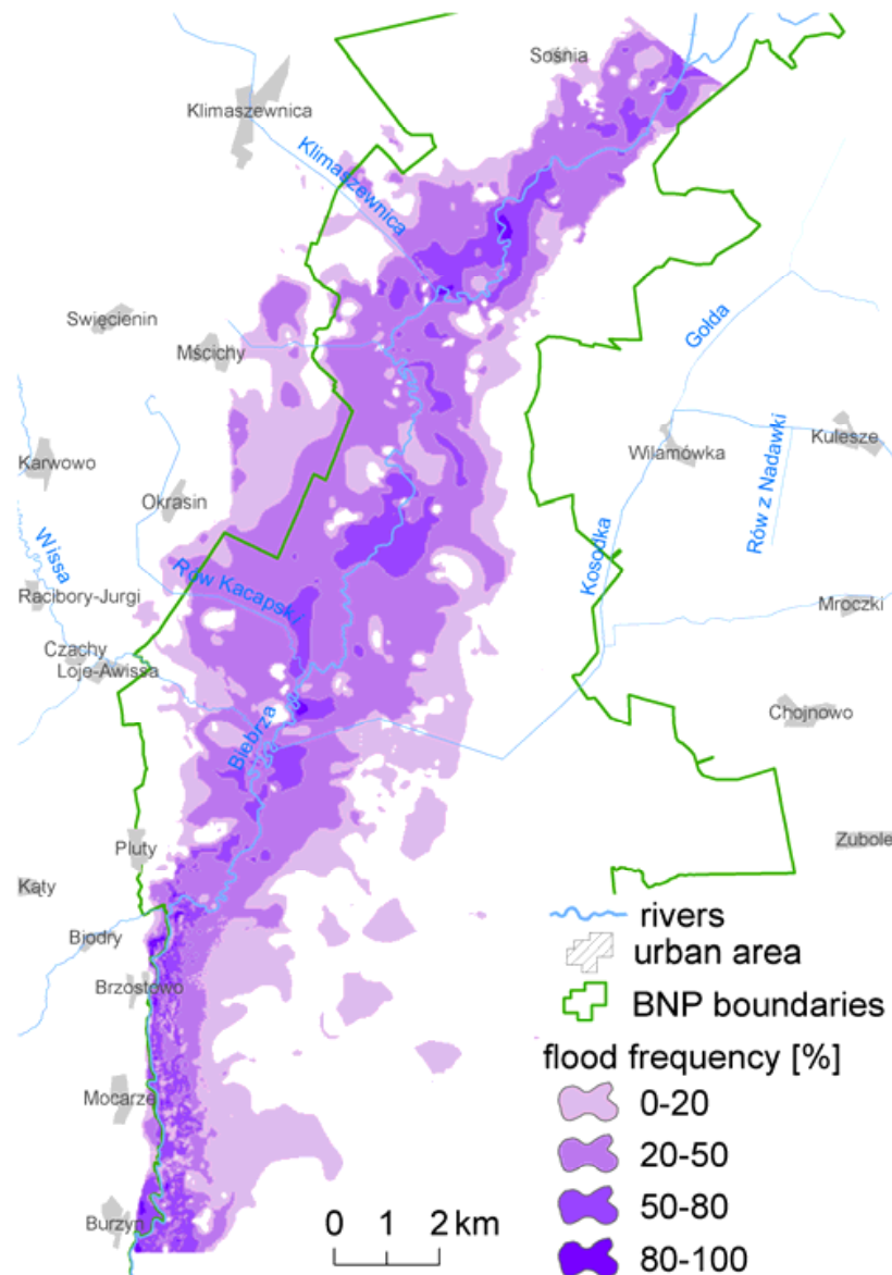
Fig. 9. Example of fluvio-genetic model results presenting of long-term annual mean flood frequency on Biebrza Lower Basin in the vegetation season (February-September) in the period 1961 till 1996 (Chormanski et al., 2009b)
