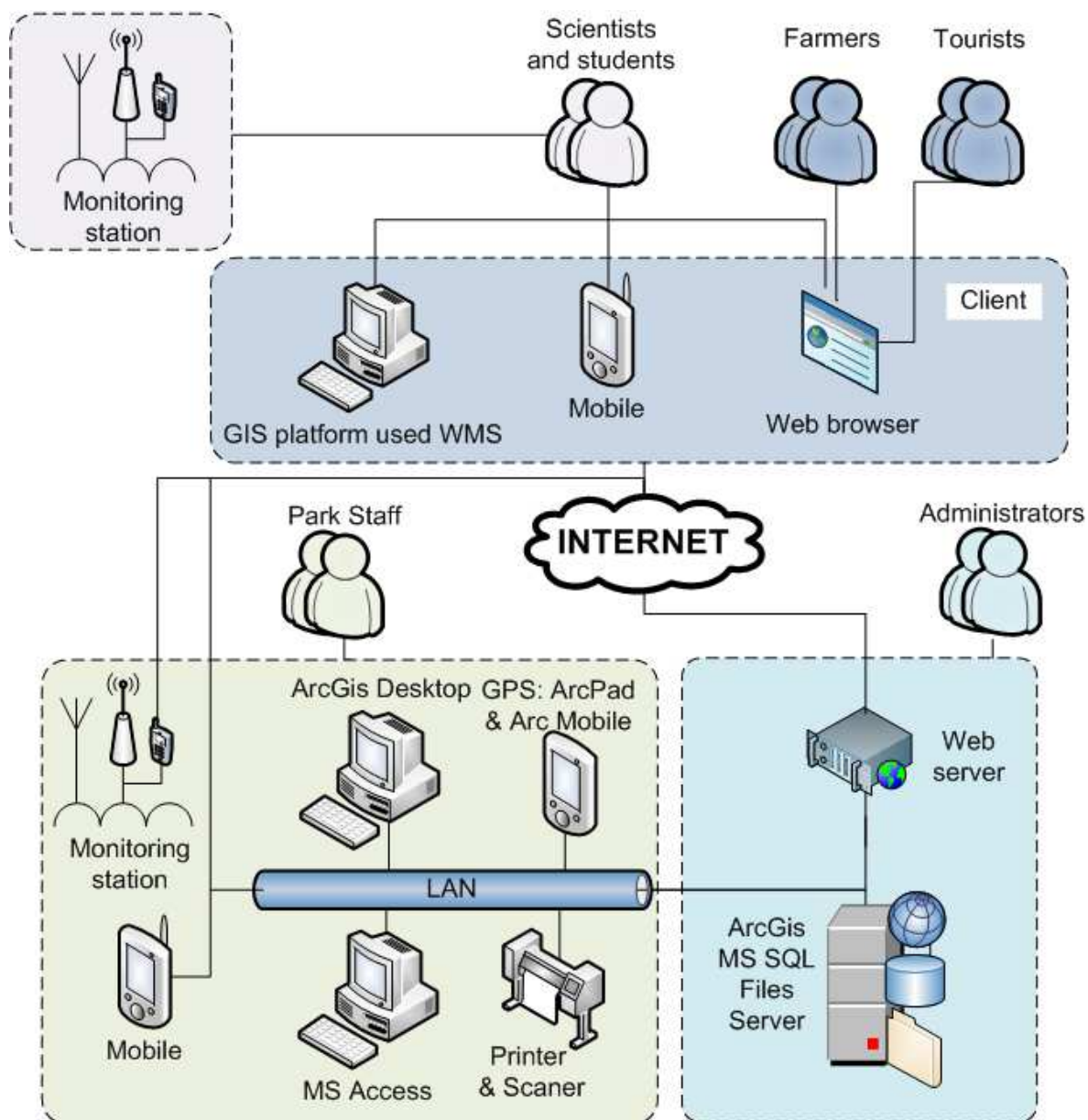
Fig. 2. Communication flow diagram for DSS
