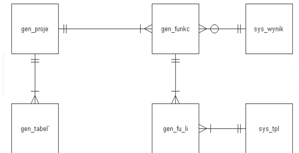
Fig. 3. The part of ERD (simplified Martin’s notation) diagram for the system tables.
