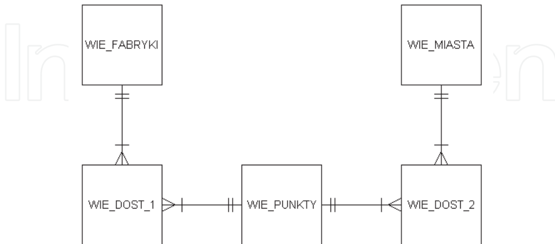
Fig. 7. The part of ERD (simplified Martin’s notation) diagram for questions parameters tables
