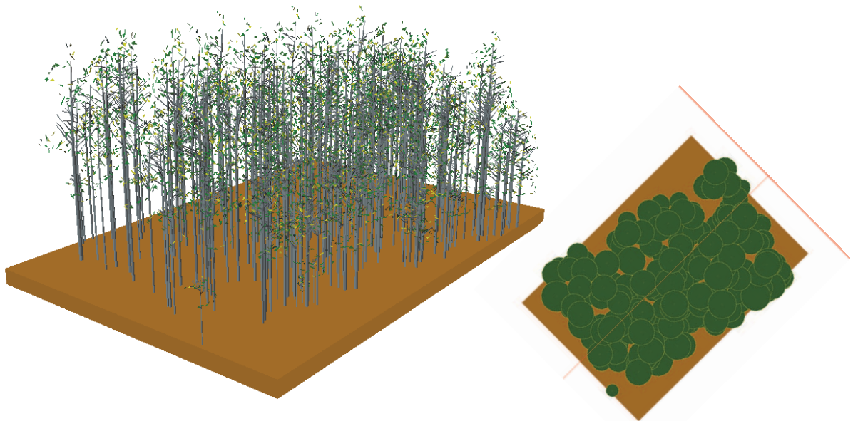
Fig. 1. 3D visualisation of research plot in age of 11 years
