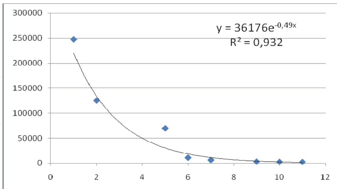
Fig. 2. Population density (No. of trees per hectare). development during succession
