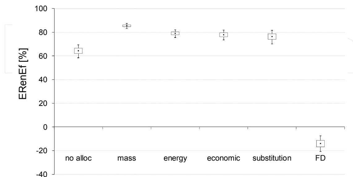
Fig. 3. RO life-cycle ERenEf results: scenario and parameter uncertainty
