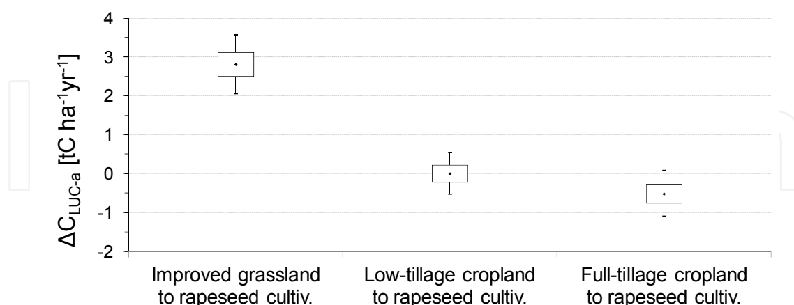
Fig. 2. Soil carbon exchange associated with LUC scenarios for Rapeseed Oil. The boxes show the interquartile range, the mark is the median and the ends of the whiskers are the 5 th and 95 th percentiles. Same notation is used in figs. 3 and 5
