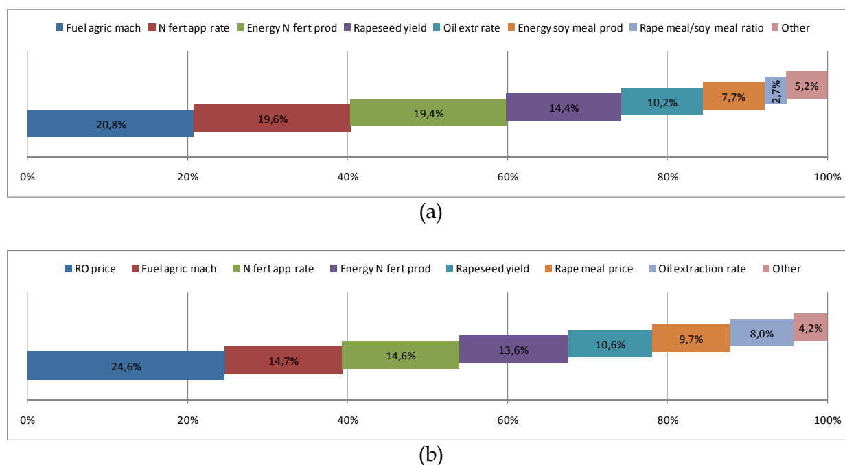
Fig. 4. Contribution of input data to the variance of RO life-cycle ERenEf: (a) substitution method; (b) economic allocation
