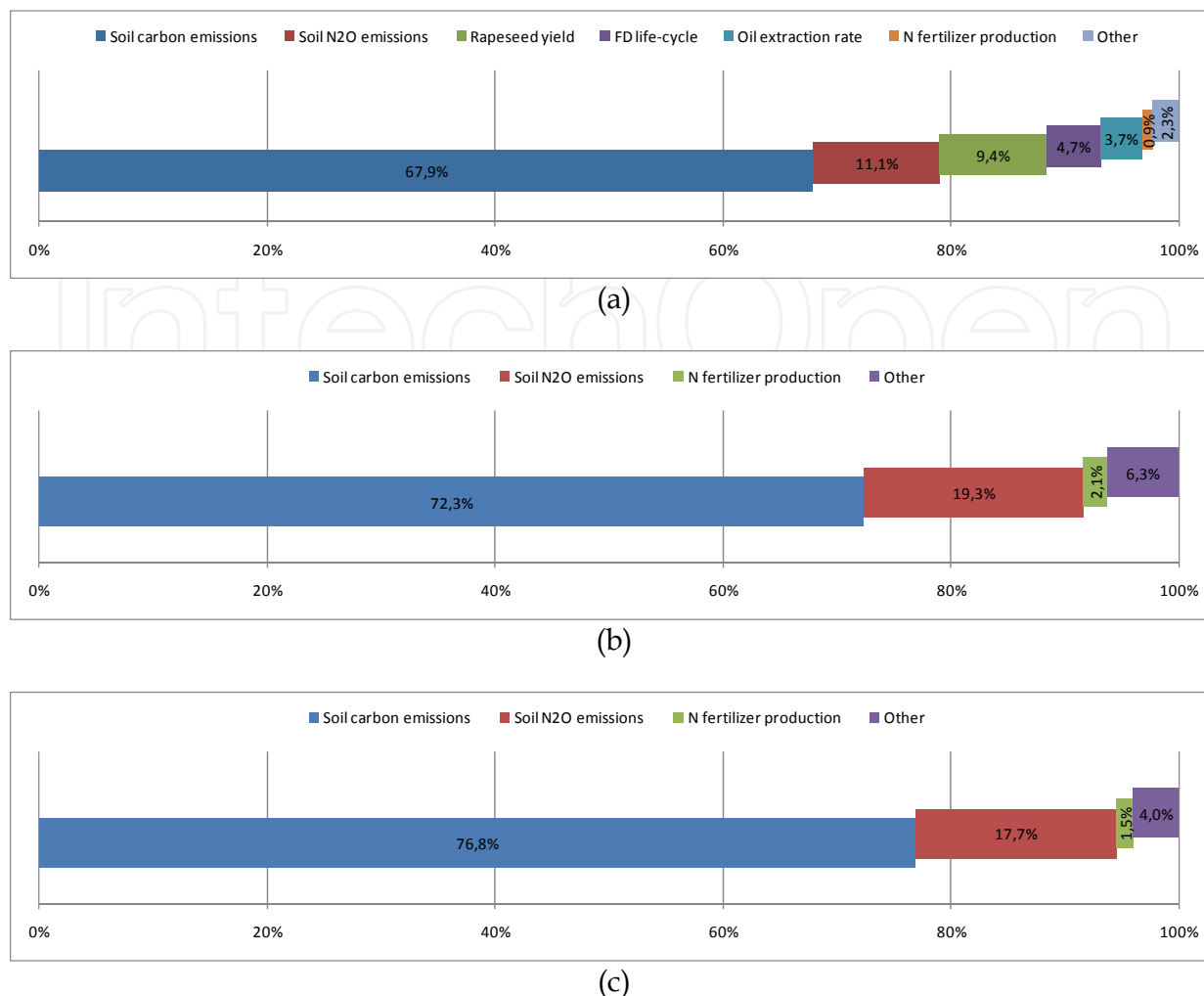
Fig. 6. Contribution of input data to the variance of RO life-cycle GHG emission savings (substitution method). Land use change scenarios: (a) improved grassland to rapeseed cultivation; (b) low-tillage cropland to rapeseed cultivation; (c) full-tillage cropland to rapeseed cultivation
