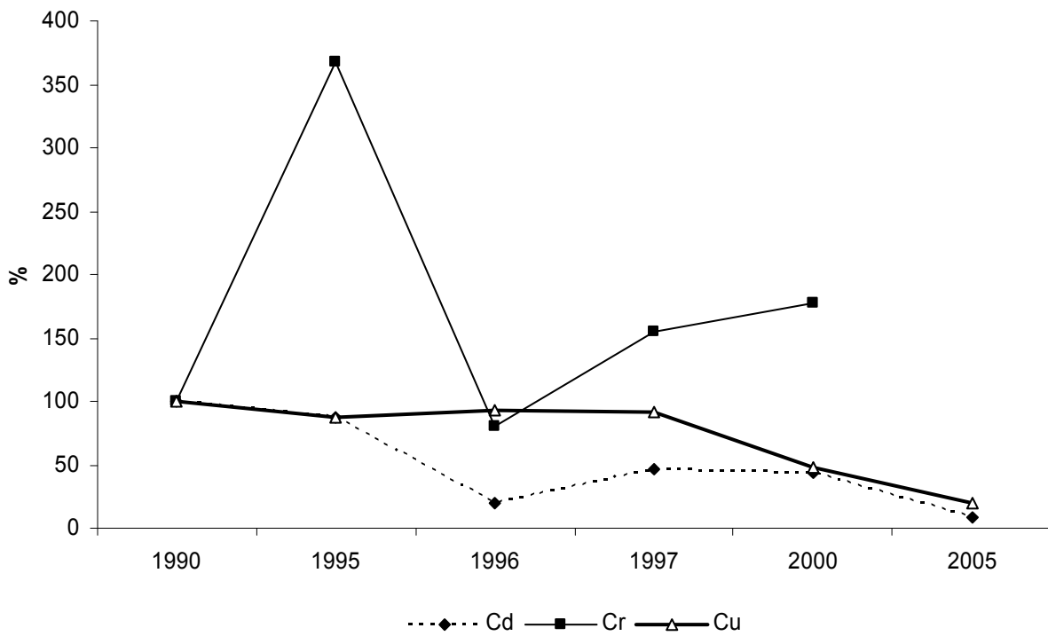
Fig. 1. Concentration of Cd, Cr and Cu (in % of average) in mosses for Slovakia in all survey years
