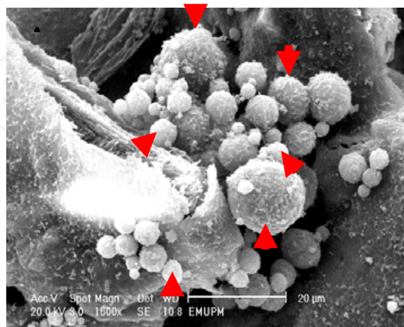
Fig. 7. ESEM microphotographs of rabbit osteoblasts cultured on different scaffolds for 3 days (arrowhead) and 7 days (arrow) show the structure of the osteoblast cells on scaffold 262 (bars = 20 \mu m)
