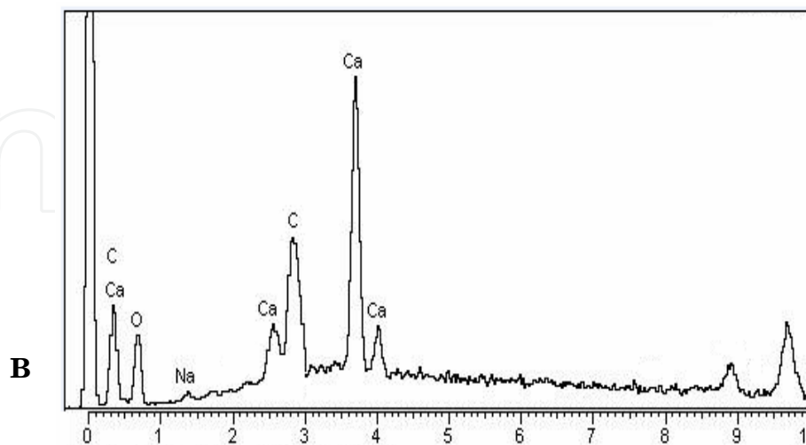
Fig. 10. SEM microphotograph (A) shows the osteoblasts grown on bioceramic scaffolds at 19 days of dynamic proliferation, (B) spectrum 1 depicts the extra cellular matrix and spectrum 2 the calcium carbonate as determined by EDX analysis
