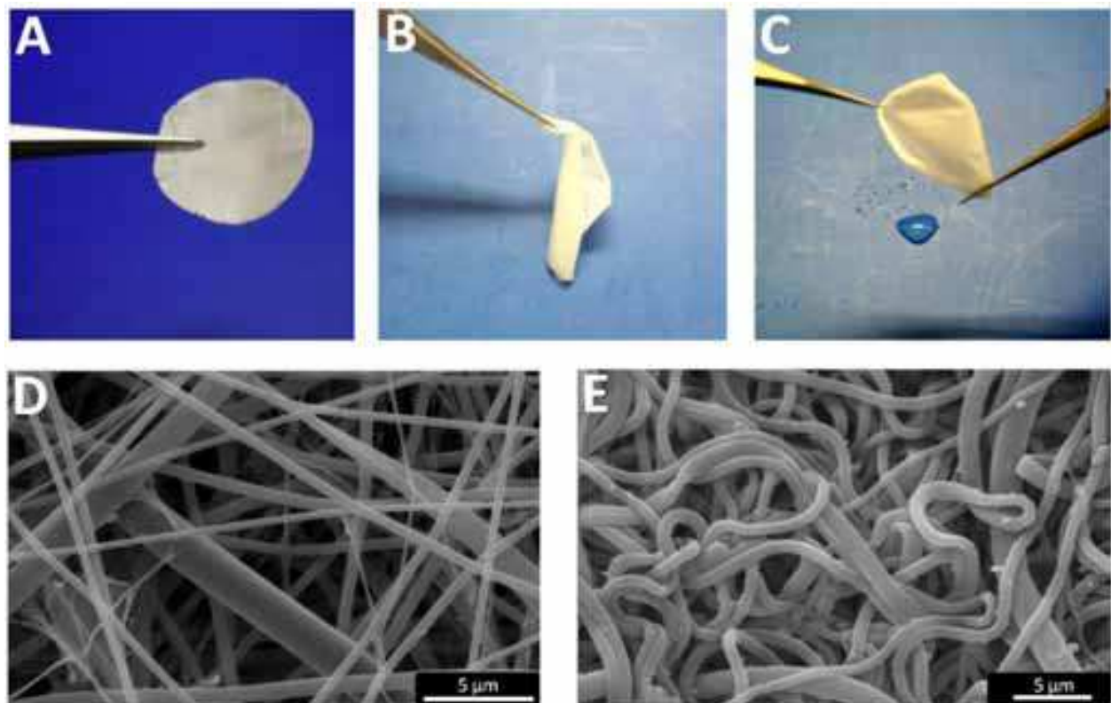
Fig. 5. Synthetic elastin electrospun materials.
