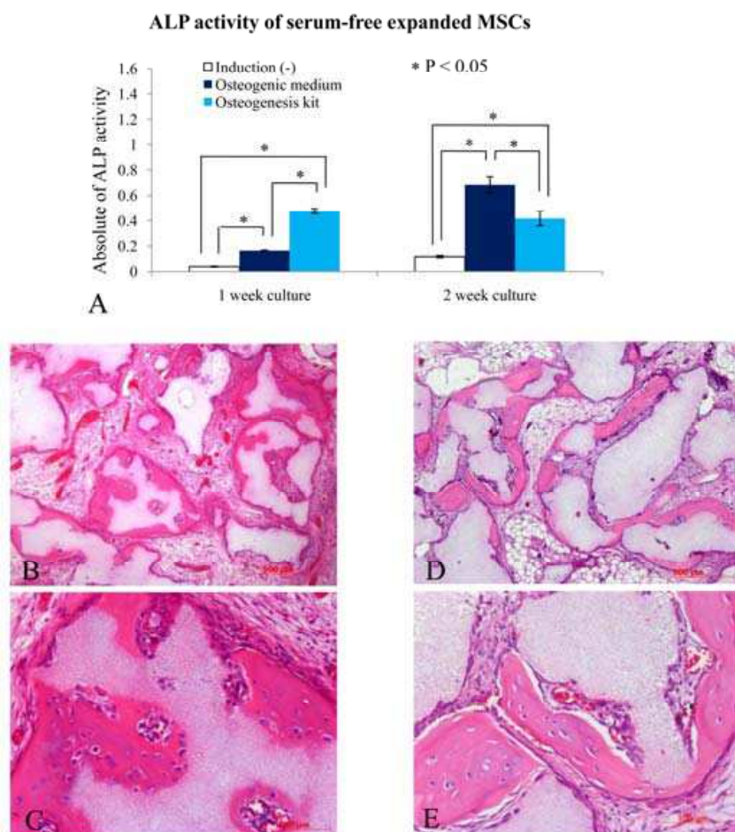
Fig. 1. Osteogenic abilities of serum-free expanded BMSCs after osteogenic induction with either osteogenic medium or osteogenesis kit (From Agata et al. , 2009 with permission)
