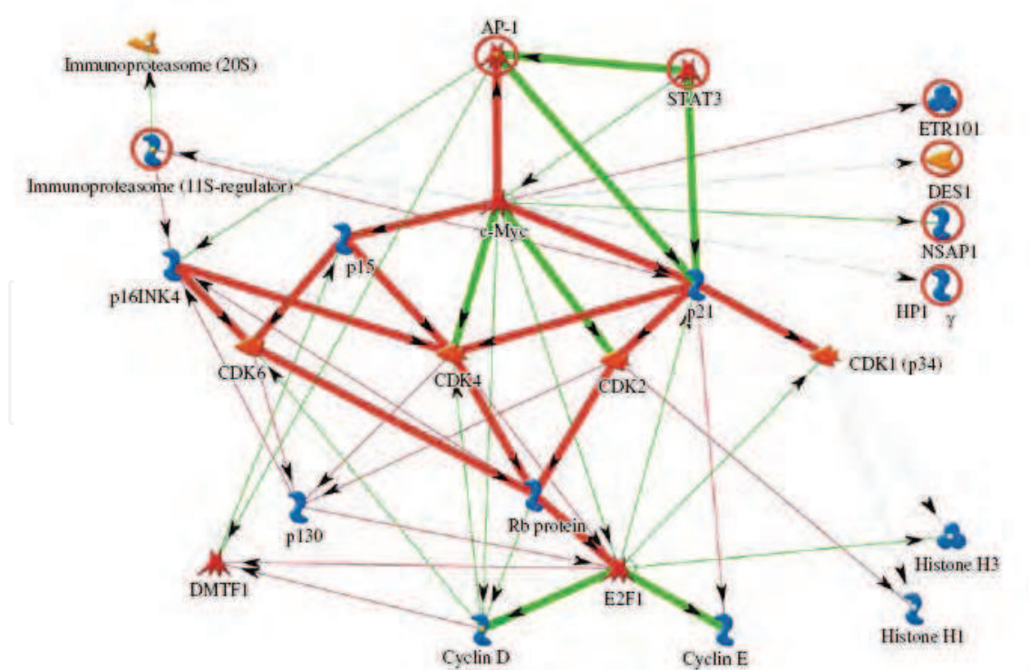
Fig. 3. Detail of the gene network describing cell cycle control. Green arrows indicate activation of the corresponding elements; red arrows, inhibition; and red circles, genes from the list.
