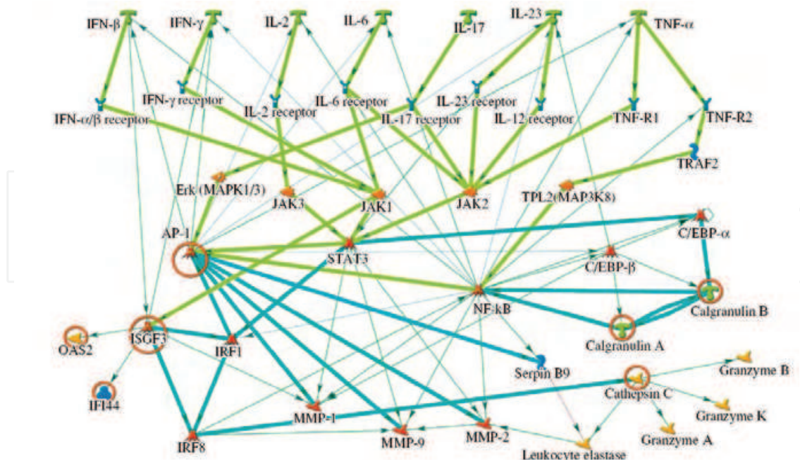
Fig. 2. Detail of the gene network describing inflammatory response. Green arrows indicate activation of the corresponding network elements, from the level of cytokines to transcription factors; light blue arrows, the activation of effector genes by transcription factors; and red circles, genes from the list.
