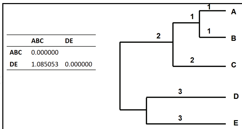
Fig. 7. The updated distance matrix and clustering of OTUs after the 3 rd iteration of UPGMA. Numbers on the branches indicate branch lengths, which are additive.
