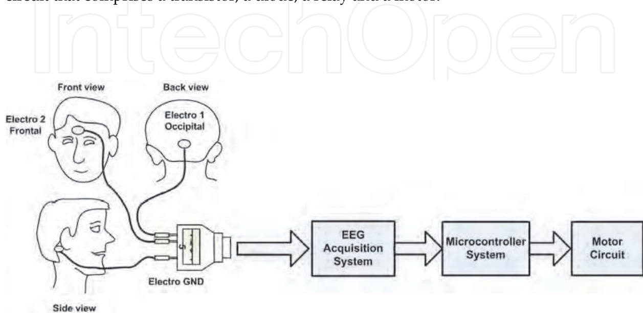
Fig. 9. Block diagram of EEG based fan system.
