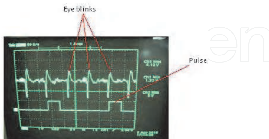
Fig. 15. Pulses generated at the output of PIC microcontroller when three eye blinks are detected. [Wahy et al, 2010]
