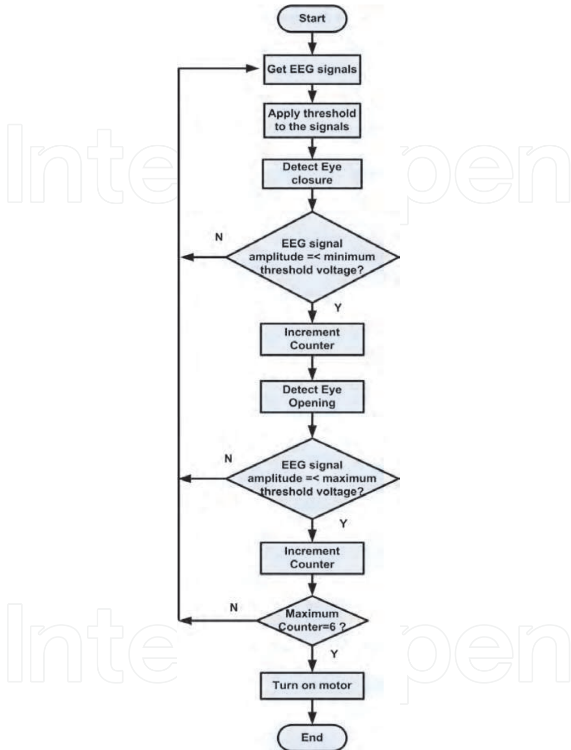
Fig. 12. Process of activating a motor using eye blink detected from EEG.
