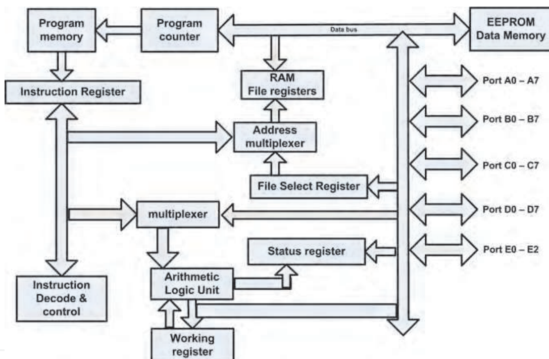
Fig. 8. Internal architecture of PIC16F877A microcontroller.
