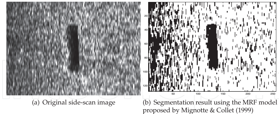
Fig. 7. MRF segmentation
