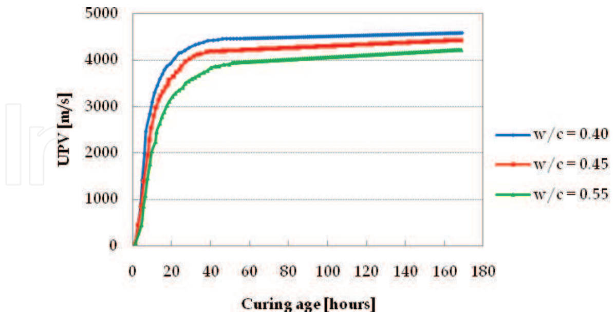
Fig. 12. Effect of the w/c ratio on UPV (Ye et al., 2004)
