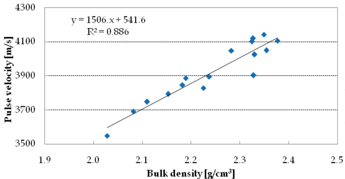
Fig. 11. Correlation plot between the bulk density and the pulse velocity (Panzer et al., 2008)
