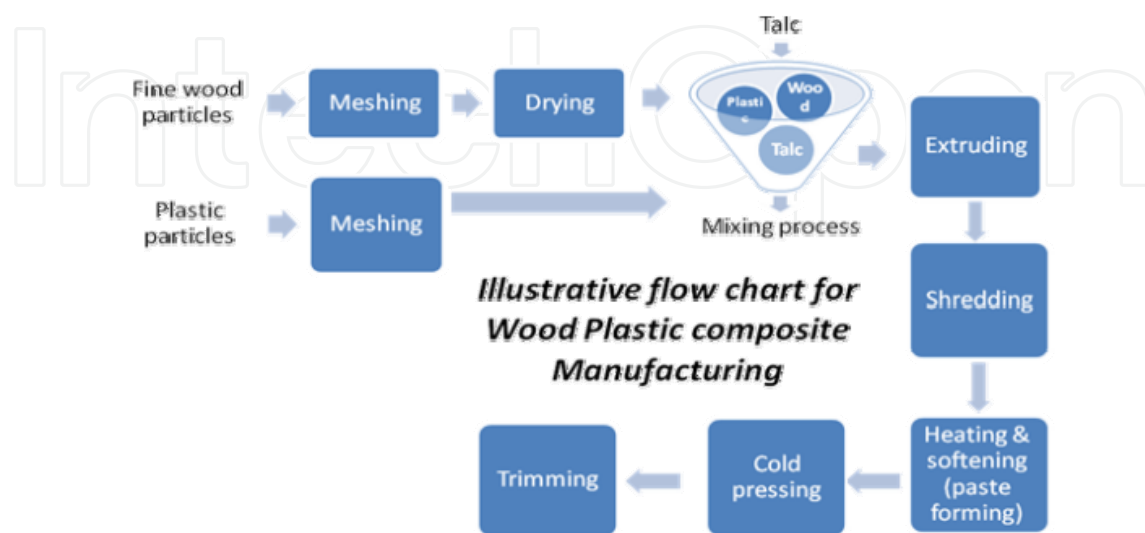
Fig. 1. Illustrative process flow chart of WPC manufacturing
