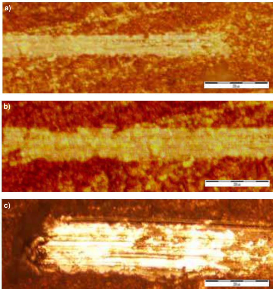
Fig. 27. Characteristic images of wear tracks of worn surface of sample after „scratch test” obtained using optical microscope (magnification 50 x): a) F= 10\ \text{N} , b) F= 20\ \text{N} , c) F= 25\ \text{N}
