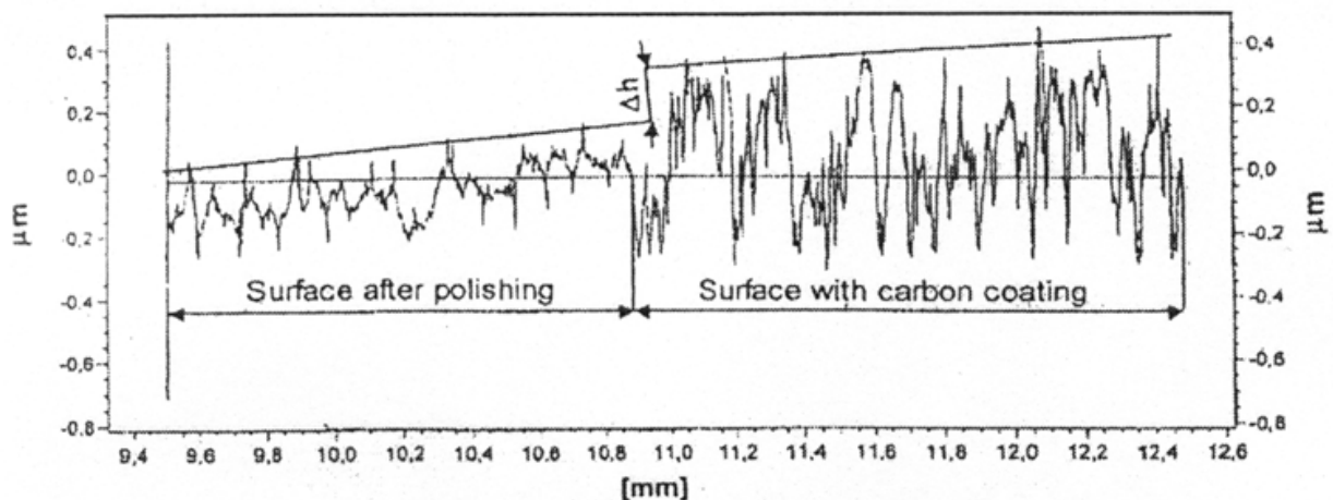
Fig. 11. Results of measurements of the thickness of carbon coating deposited on magnesium alloy AZ31 carried out by the method of direct profilography; the thickness of carbon coating ( \Delta h ) of 220 nm
