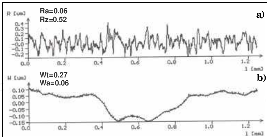
Fig. 14. Profilograms of roughness (a) and waviness (b) in 2D configuration of AZ31 magnesium alloy surface with manufactured carbon coating
