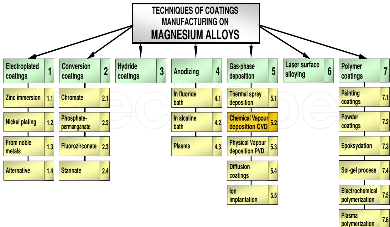
Fig. 2. Techniques of coatings manufacturing on magnesium alloys
