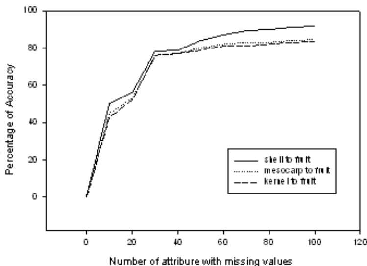
Fig. 3. Comparison of most observed attribute in missing values
