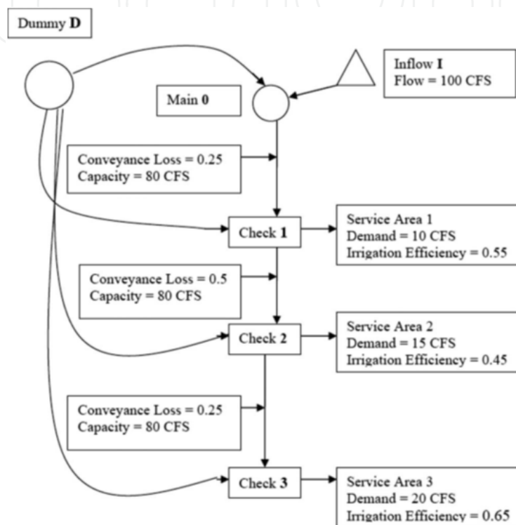
Fig. 9. Hypothetical Irrigation Network (NMISC, 2006)
