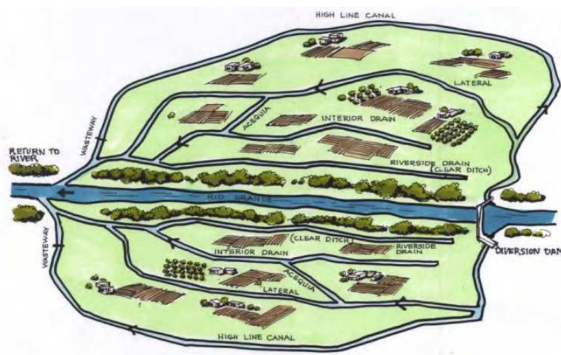
Fig. 4. Representation of MRGCD Irrigation System
