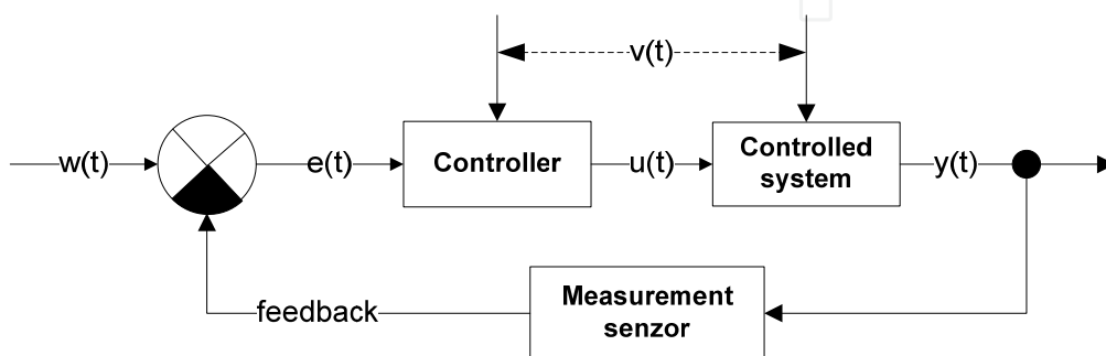
Fig. 5. Control loop
