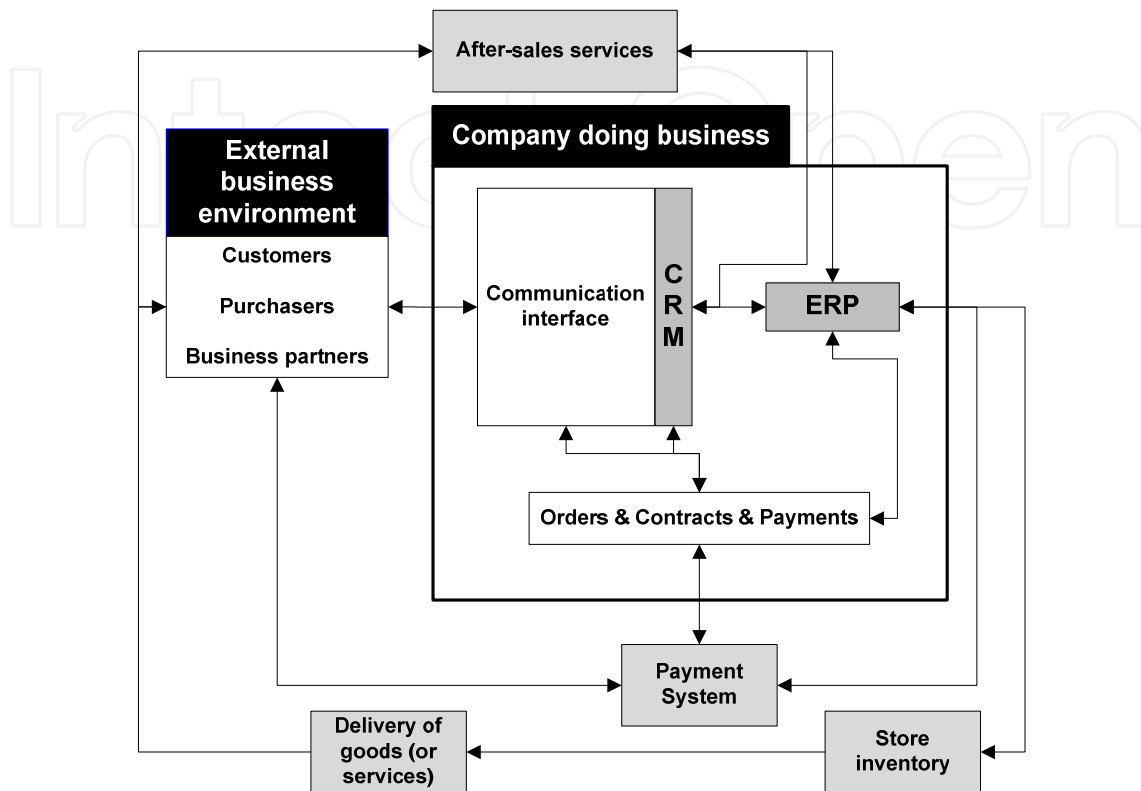
Fig. 1. E-commerce system
