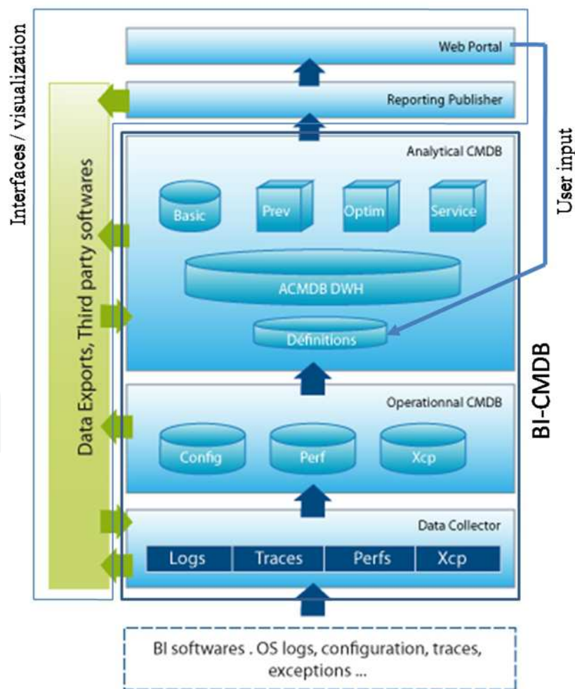
Fig. 1. The SP2 BI-CMDB simplified schema
