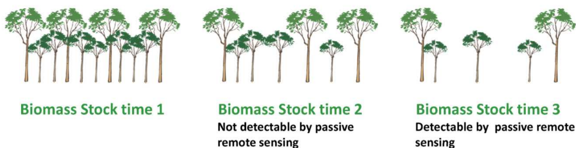
Fig. 1. Different status of forest degradation and potential of detection by passive remote sensing techniques (Baldauf et al., 2009)
