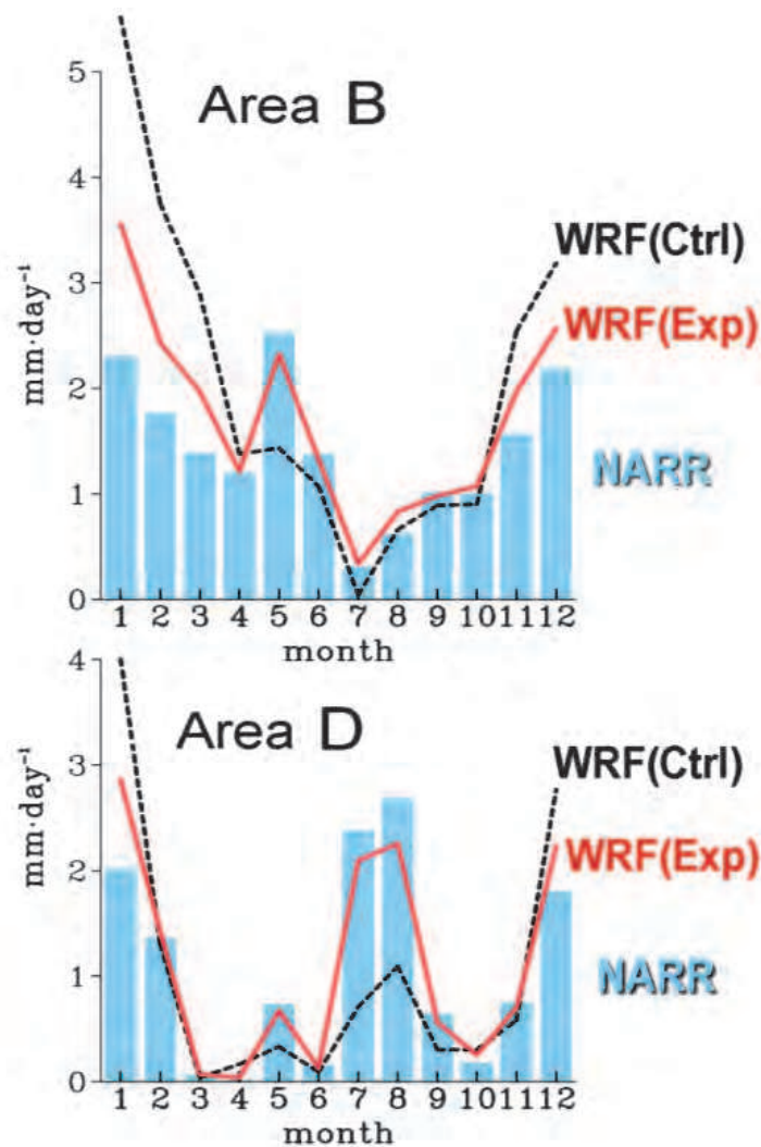
Fig. 7. Monthly precipitation of 2008 in areas B and D from the observation (bars), WRF(Ctrl) (black dashed line), and WRF(Exp) (red solid line). The observation here uses the North American Regional Reanalysis (NARR).
