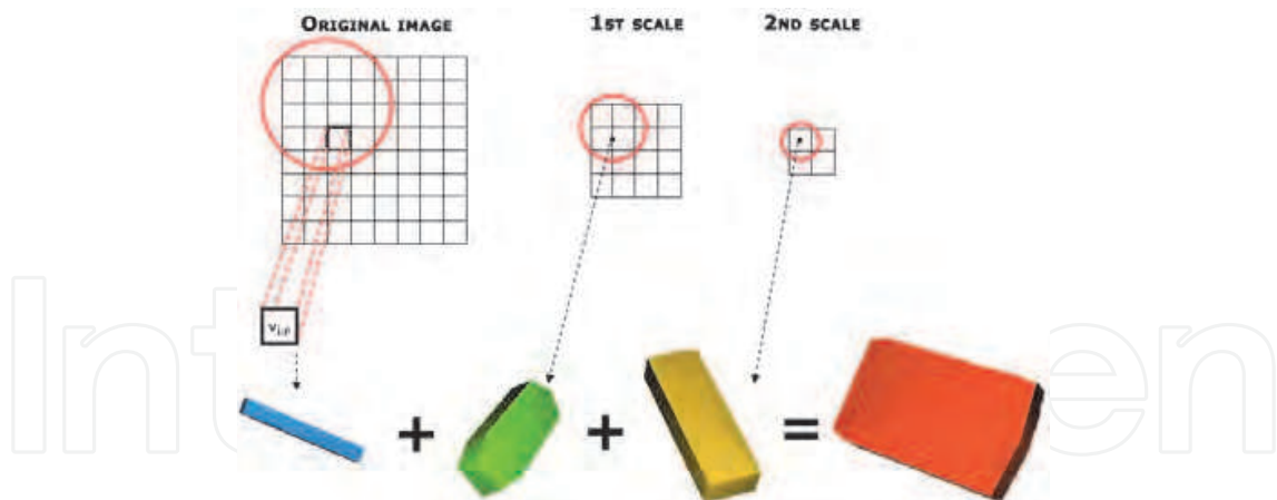
Fig. 15. A tensor is computed for each pixel in original image by a weighted sum of corresponding tensors in each scale. In this example, two wavelet decompositions are performed.
