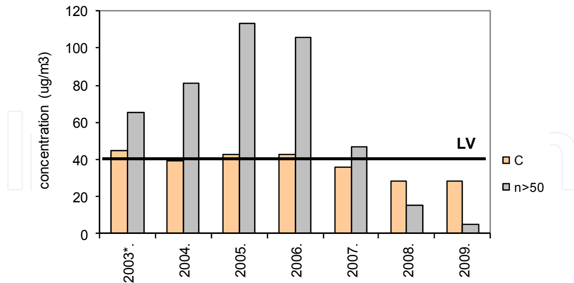
Fig. 8. Annual means (C) of PM 10 measured with analyzer (n>50- number of exceedances of LV d =50 μg m -3 )
