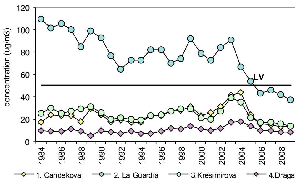
Fig. 2. Annual mean concentrations of black smoke (limit value LV=50 µg m -3 )
