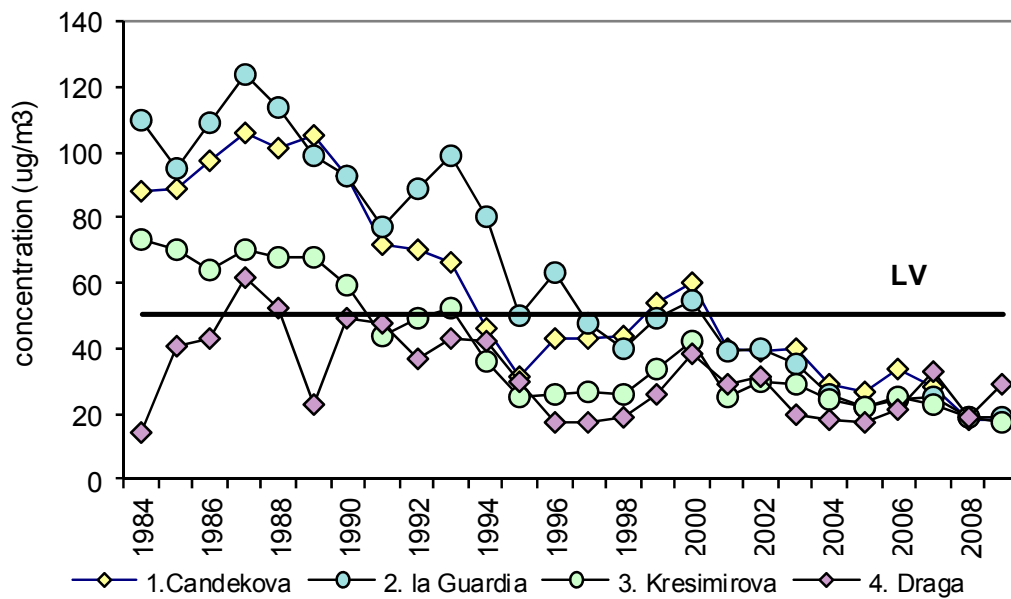
Fig. 1. Annual mean concentrations of sulphur dioxide (limit value LV=50 µg m -3 )
