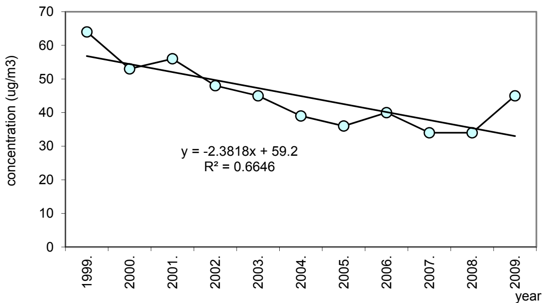
Fig. 6. Annual mean concentrations of ozone
