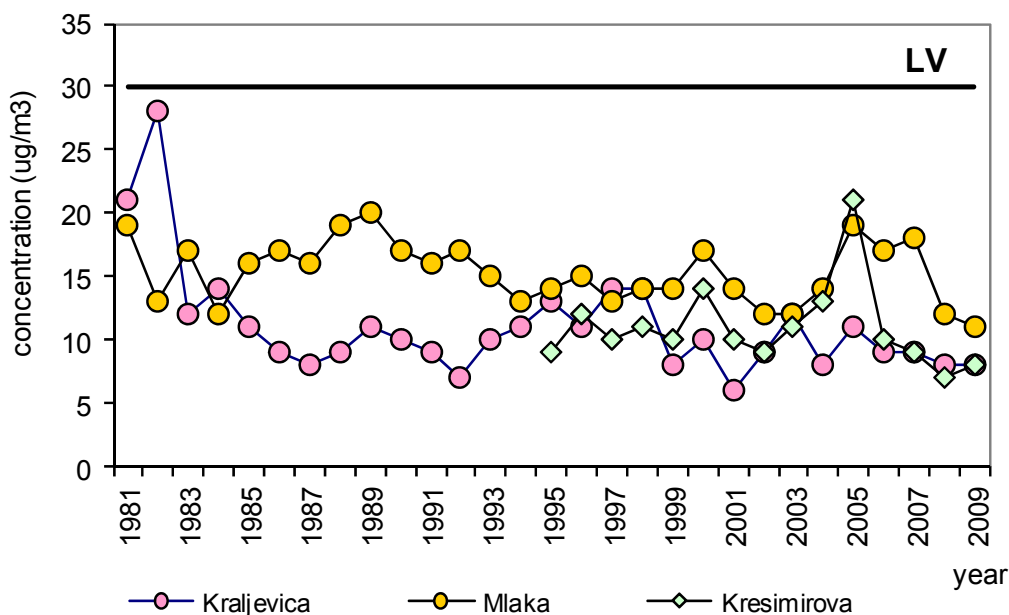
Fig. 4. Annual mean concentrations of ammonia (limit value LV=30 \mu\text{g m}^{-3} )
