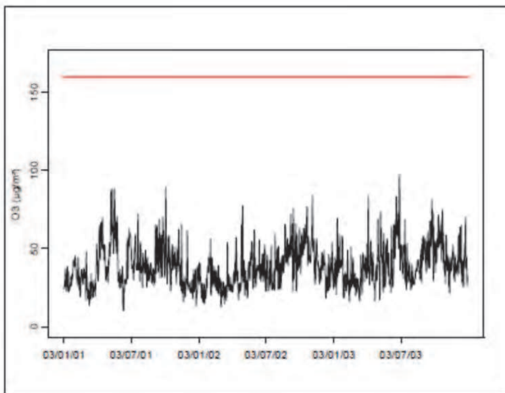
Fig. 10. Daily average concentrations of O 3
