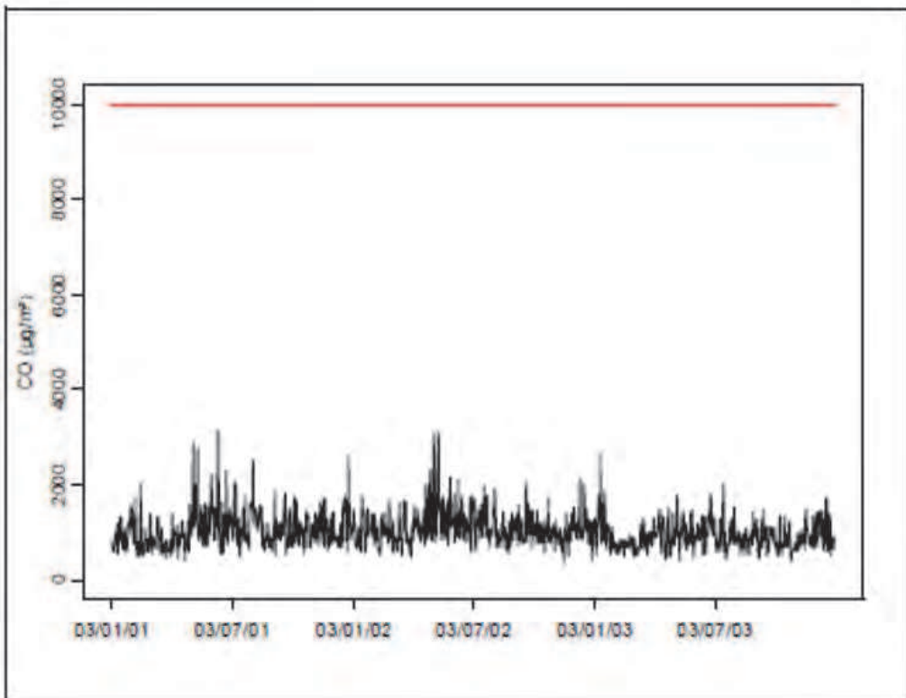
Fig. 9. Daily average concentrations of CO
