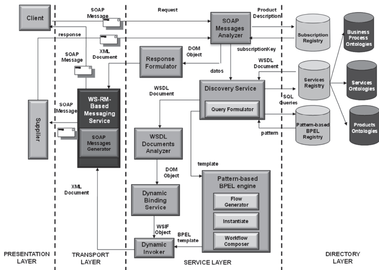
Fig. 4. The middleware-oriented integrated architecture for e-procurement
