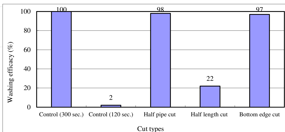
Fig. 6. Washing efficacy of the different cut types
