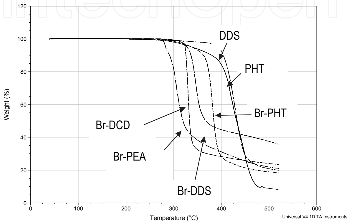
Fig. 1. TGA of epoxy-system based on Diglycidyl ether of bisphenol A or Diglycidyl ether of tetrabromobisphenol A (Br) crosslinked using different hardeners; DDS: Diaminodiphenylsulphone; DCD: Dicyandiamide; PEA: Polyethylene-polyamine, PHT: Phthalic anhydride. (20°C/min, Nitrogen)
