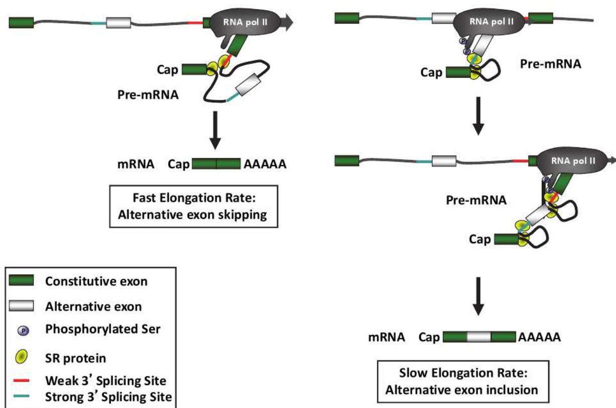
Fig. 2. Kinetic model for co-transcriptional splicing.
