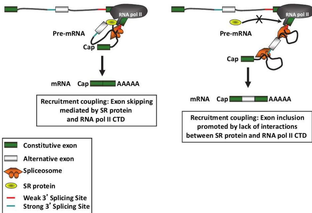
Fig. 4. Recruitment model for co-transcriptional splicing.
