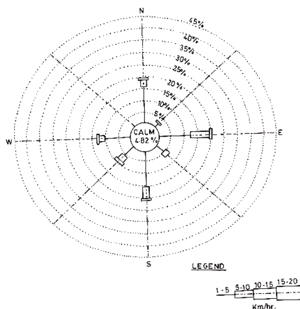
Fig. 1. Wind Rose Diagram of Padampur OCP
