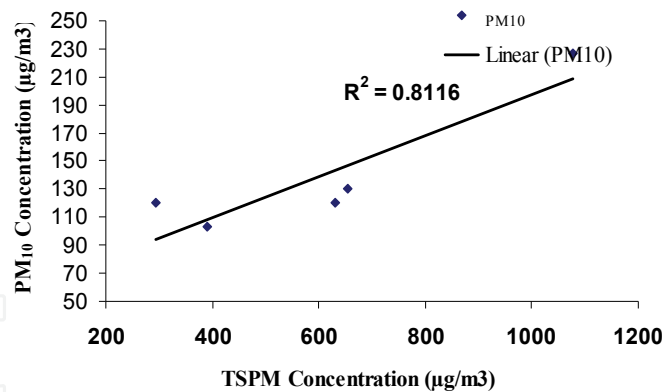
Fig. 4. Correlation between TSPM and PM 10 Concentration.
