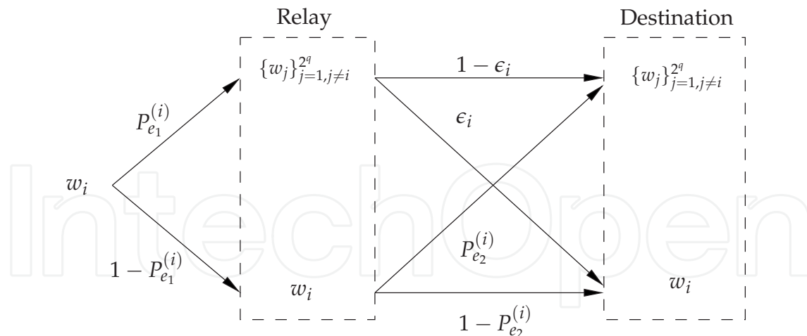
Fig. 4. Error probability transition in DF relaying.
