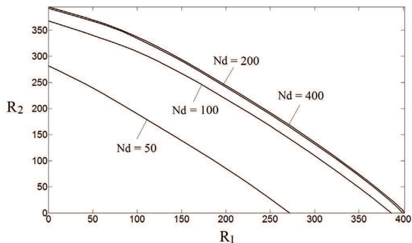
Fig. 9. Rate regions for different number of rate discretization values N_d
