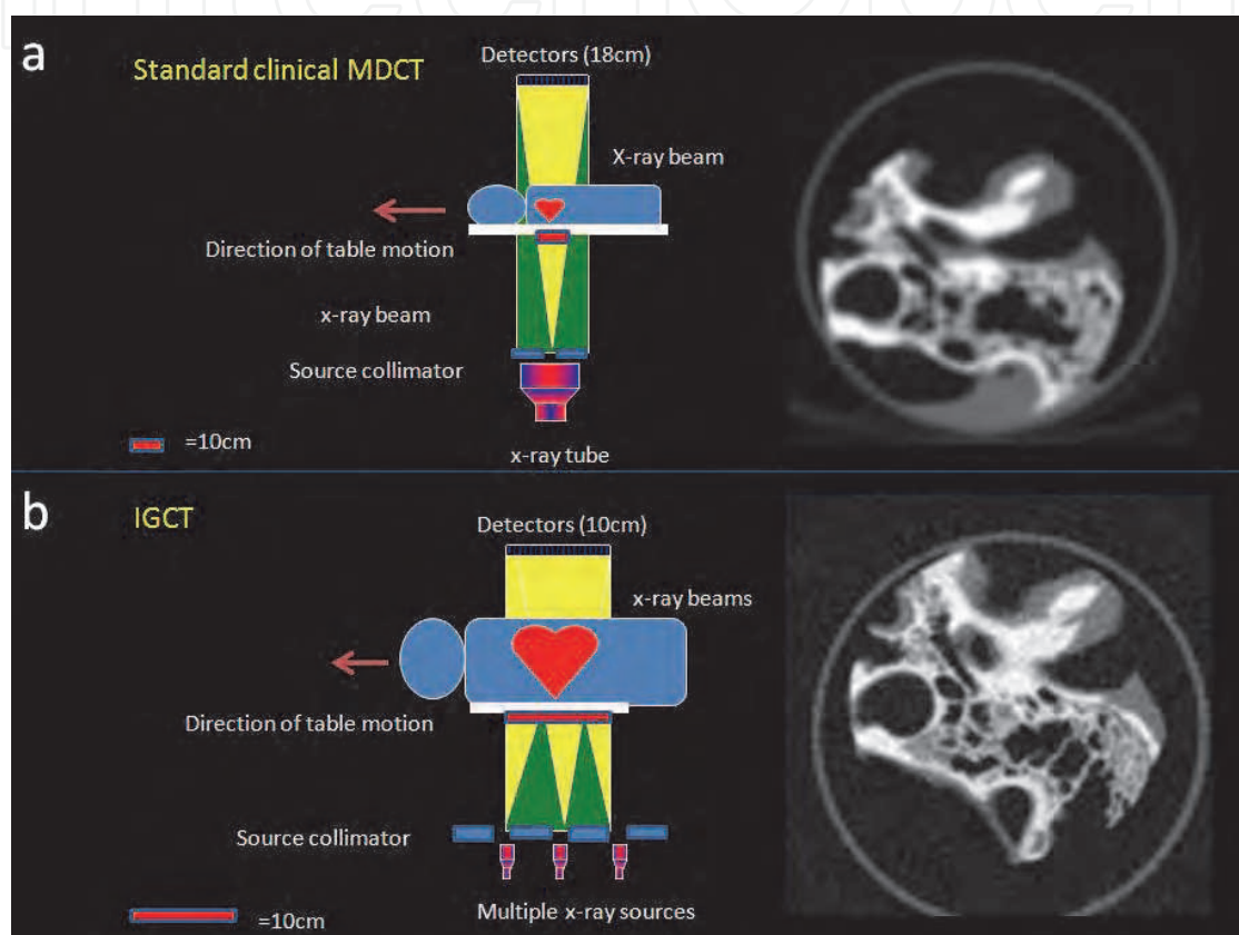
Fig. 18. Standard MDCT (a) requires an 18cm detector array when scanning a 10cm region of interest (due to cone beam) introducing artefacts at beam edges. Inverse Geometry CT (IGCT) (b) uses multiple x-ray sources and only requires a 10cm detector array for a 10cm region of interest, reducing detector size and weight, reducing cone beam artefact and producing greater signal to noise ratios for reduced radiation exposure.
