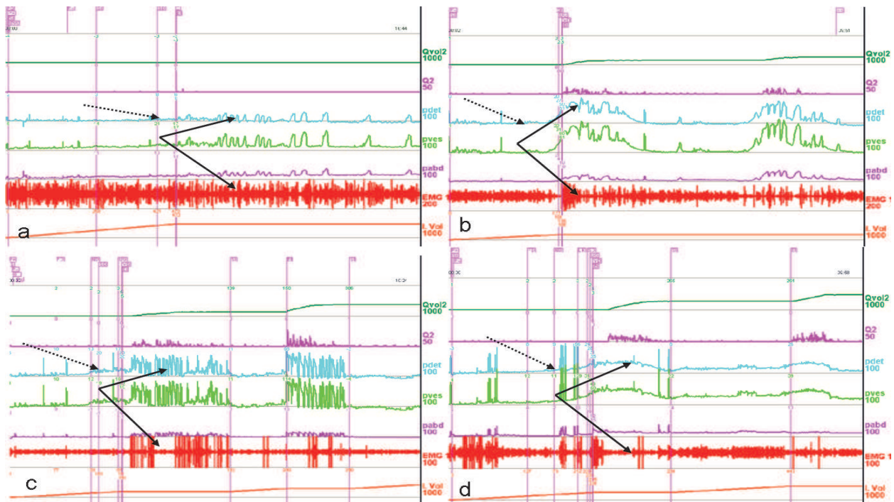
Fig. 12. Comprehensive urodynamic tracings of female patients with DUA-NC and the efficacy of LFE were displayed. The dashed arrows indicate normal compliance and solid arrows indicate the state of the detrusor contractility and the sphincter relaxing ability during voiding phase. (a) A women aged 32 years old, complained of chronic retention for 2 weeks due to iatrogenic reason, and her detrusor was still underactive when more than 500 ml saline was infused into the bladder. (b) After LFE, her detrusor function recovered, sphincter overactivity improved and got rid of catheterization thereafter. (c) A female patient, 52 years old, complained of urgency and frequency for two months, urodynamic study showed DUA and sphincter overactivity before LFE. (d) After the procedure, detrusor became contractile and sphincter overactivity still remained. EMG, electromyogram; I. Vol, infused volume; Pabd, abdominal pressure; Pdet, detrusor pressure; Pves, vesical pressure; Q, flow rate; Qvol, uro volume.
