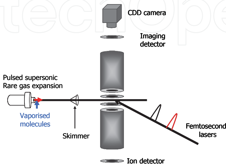
Fig. 3. Experimental setup.
