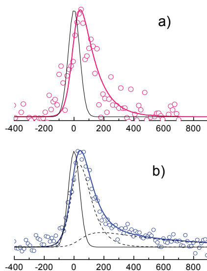
Fig. 12. Time evolution of vitamin B 12 (a), while scanning the pump/probe delay (400/800 nm) compare to the time evolution of CoTPP (b). The experimental points are fitted by the solid line following a three level model. The contribution of each component is represented by dotted curves; the dashed curve indicates the cross correlation of the pump and probe pulse.
