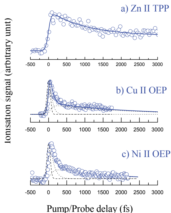
Fig. 8. Ion signals of (a) [\text{ZnTPP}]^+ , (b) [\text{CuOEP}]^+ and (c) [\text{NiOEP}]^+ as a function of time delay between the pump (400 nm) and the probe (800 nm)
