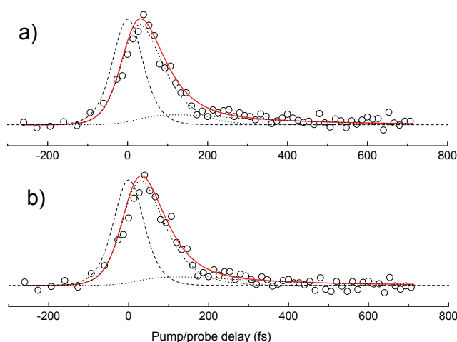
Fig. 10. Time evolution of hemin [Fe PP Cl], [Fe PP], while scanning the pump/probe delay (400/800 nm) (a) recorded at the mass of parent molecules [Fe PP Cl] + . (b) The observation is set at the mass of [Fe PP] + . The experimental points are fitted by the solid line following a three level model. The contribution of each component is represented by dotted curves; the dashed curve indicates the cross correlation of the pump and probe pulse
