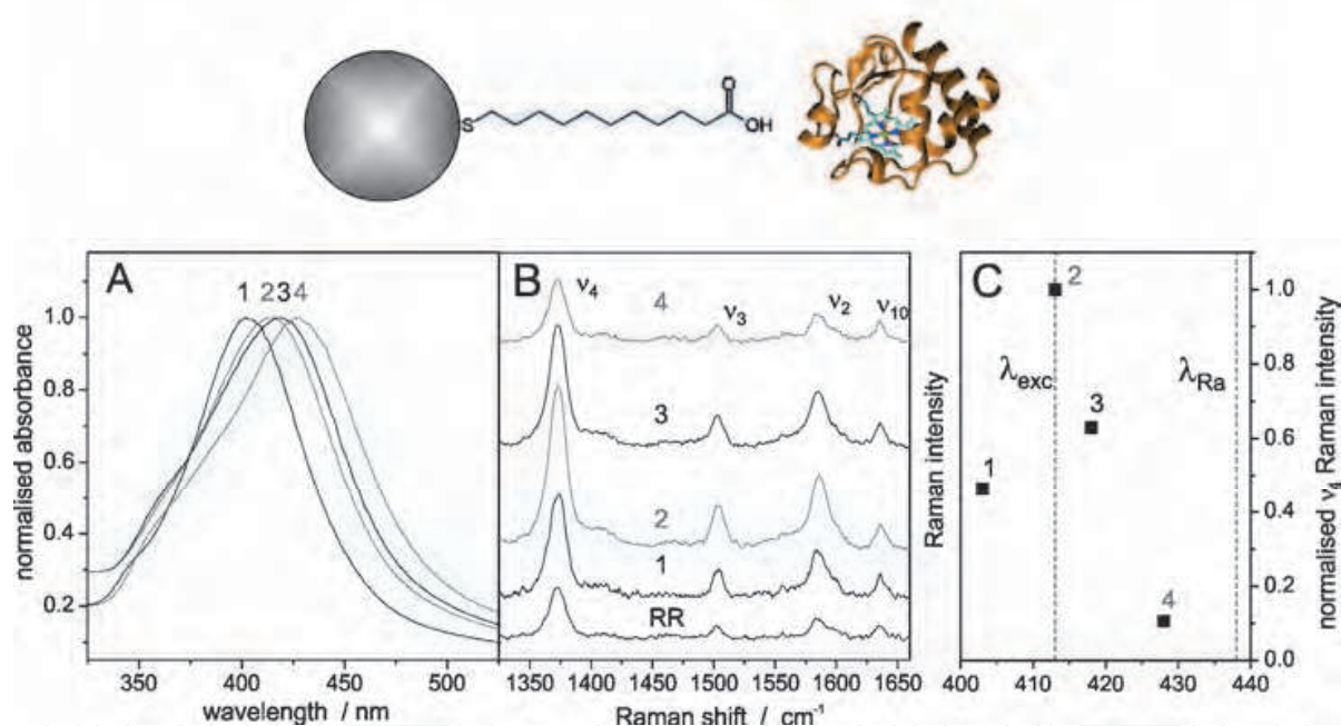
Fig. 2. (A) SPRs of MUA capped AgNPs of different average size. (B) RR and SERR spectra of Cyt c in solution and attached to NPs with different SPR maximum. (C) SERR intensity of the \nu_4 band of Cyt c on different AgNP batches as a function of their respective SPR maximum. The vertical dashed lines mark the wavelength of the laser excitation ( \lambda_{\text{exc}} ) and the Raman scattered light at the \nu_4 position ( \lambda_{\text{Ra}} ).
