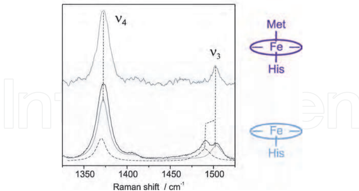
Fig. 3. RR (top) and SERR (bottom) spectrum of ferric Cyt c on AgNPs where the MUA coating is not complete. The solid grey and dashed black lines in the lower spectrum represent the respective component spectra of the native low spin and non native high spin species. On the right side the coordination of the heme in its native low spin (top) and non native high spin (bottom) state is shown schematically.
