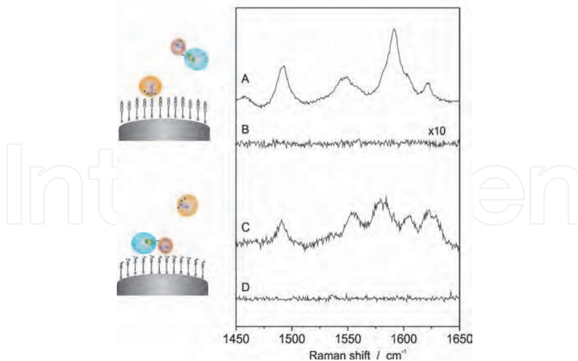
Fig. 4. SERR spectra of YCyt c (A,D) and HSO (B,C) on carboxyl (A,B) or amino (C,D) terminated SAMs. On the right side the selective binding of each protein to the respective SAM is shown schematically.
