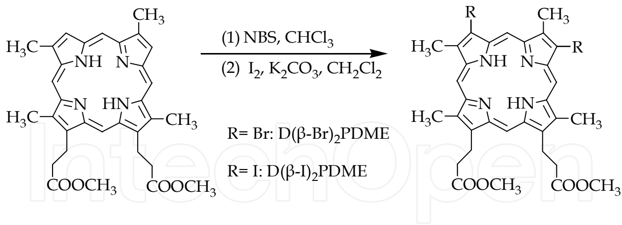
Fig. 6. Synthesis of \text{D}(\beta\text{-X})_2\text{PDME} .
