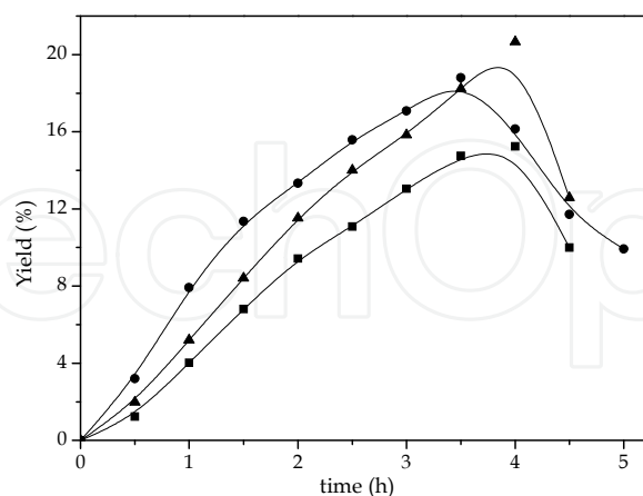
Fig. 13. Yields of cyclohexanol and cyclohexanone in the oxidation of cyclohexane catalyzed by M[D(\beta-Br)_2PDME] . Reaction conditions: cyclohexene 1000 mL, catalyst 0.02 mmol, temperature 150 °C, Pressure 0.8 MPa, Co(II)[D(\beta-Br)_2PDME] (▲); CoMn(III)[D(\beta-Br)_2PDME] (●); ClFe(III)[D(\beta-Br)_2PDME] (■).
