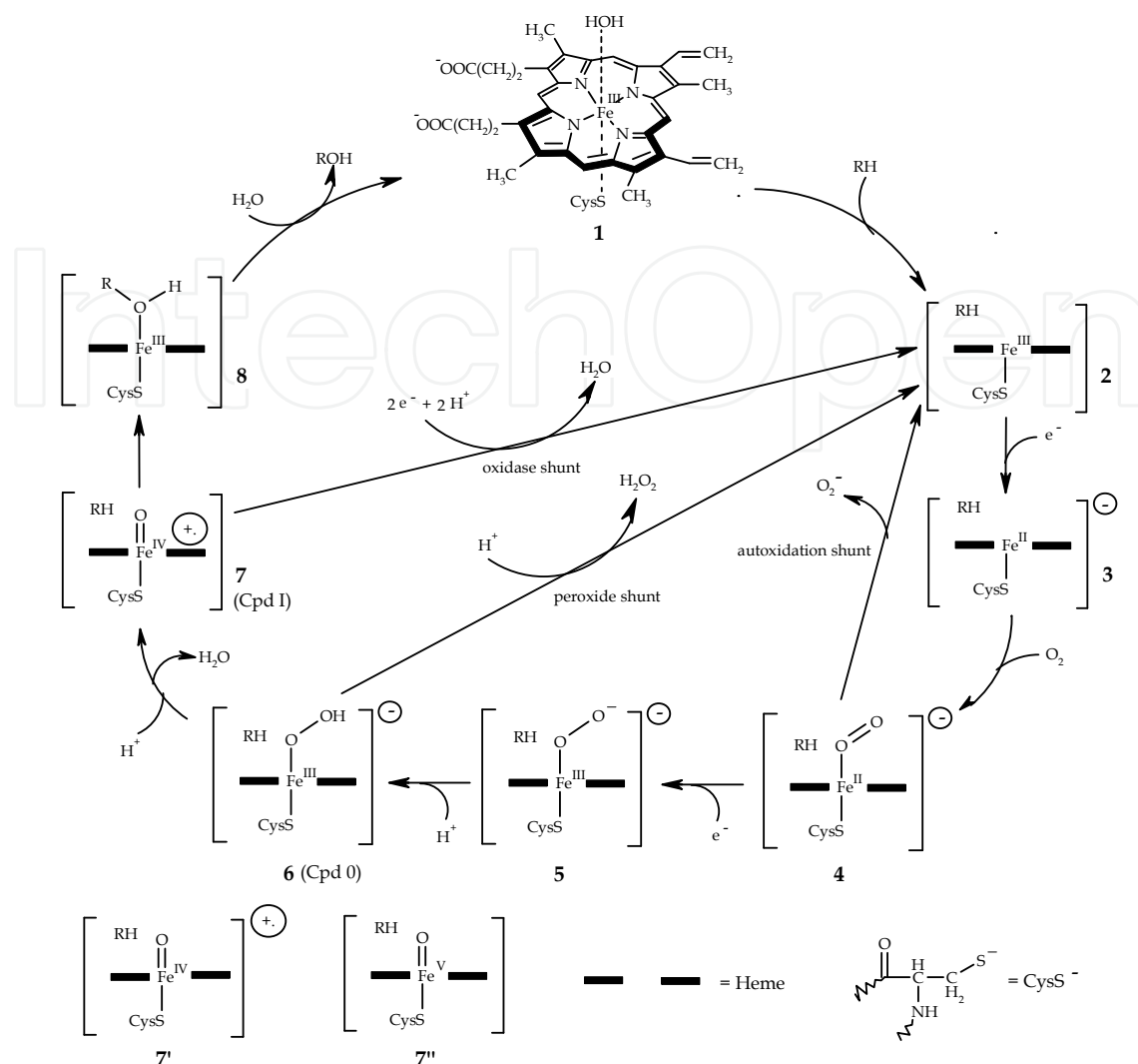
Fig. 2. Schematic representation of the catalytic cycle of cytochrome P450. RH is a substrate hydrocarbon and ROH the resulting hydroxylated product. The +• over one of the heme lines indicates that the radical cation is located on the porphyrins, whereas its placement beside the brackets indicates that the radical is located somewhere on the protein.
