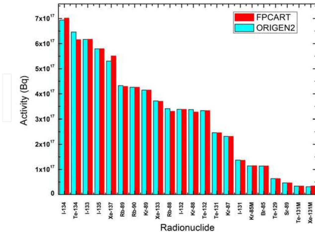
Fig. 3. For steady state operation, FPCART predicted saturation values of activities of various isotopes in PWR fuel with the corresponding computed data using the ORIGEN2 code [35]
