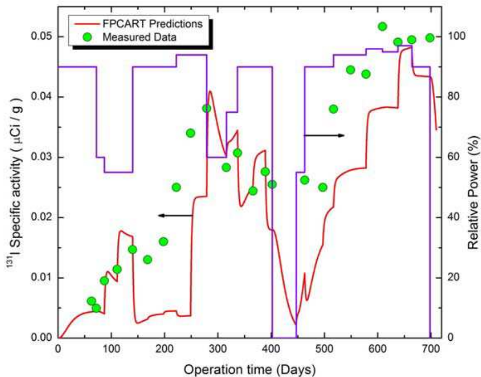
Fig. 7. For power transients, FPCART predicted values of ^{131}\text{I} specific activity variations with time compared with the corresponding experimental data for the ZORITA power plant
