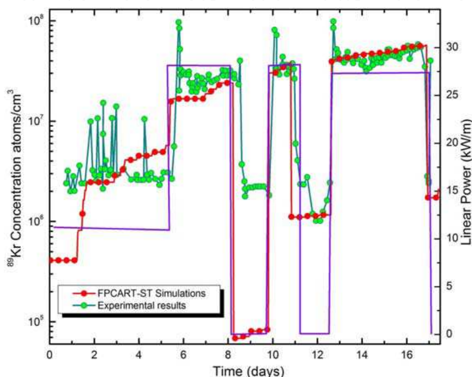
Fig. 9. For power transients, FPCART predicted values of ^{89}\text{Kr} specific activity variations with time compared with the corresponding experimental data for the EDITHMOX-1 (Unit-1) power plant [37]
