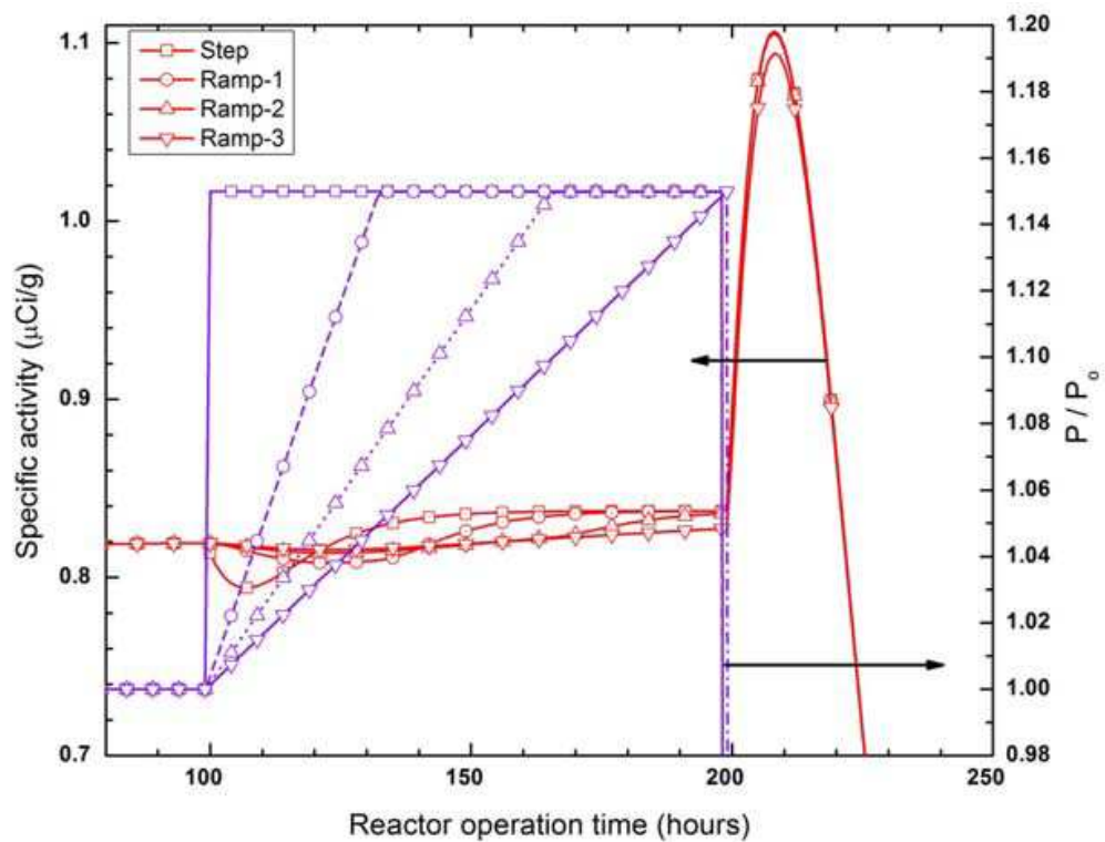
Fig. 4. FPCART simulated variation of ^{135}\text{Xe} specific activity with time for step and ramp power transients
