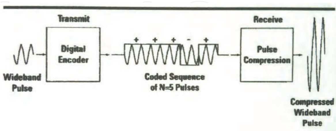
Fig. 2. Compression of wideband pulse
