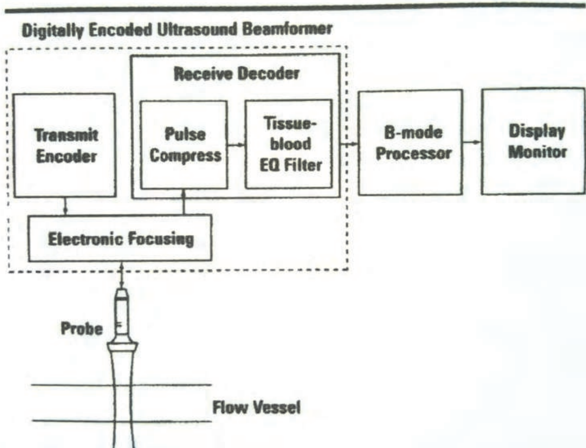
Fig. 1. Digitally Encoded Ultrasound Beamformer
