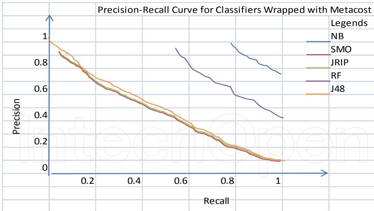
Fig. 9. Precision-Recall Curve for Various Classifiers in WEKA
