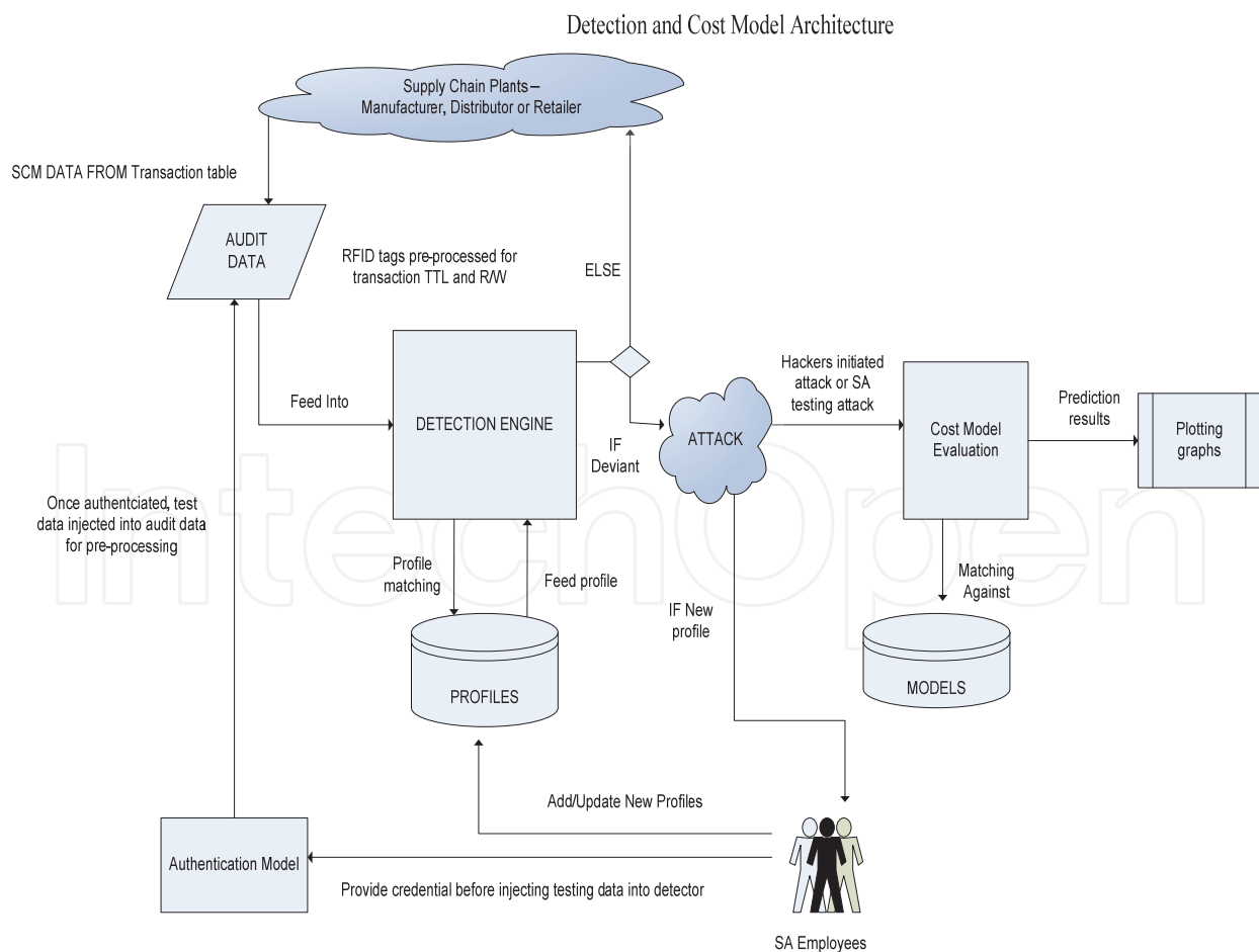
Fig. 6. Detection and Cost Model Architecture
