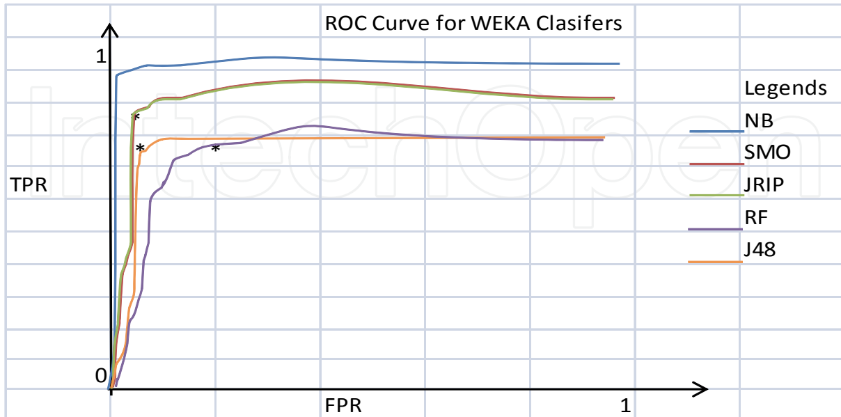
Fig. 8. ROC Curve plot for WEKA Classifiers
