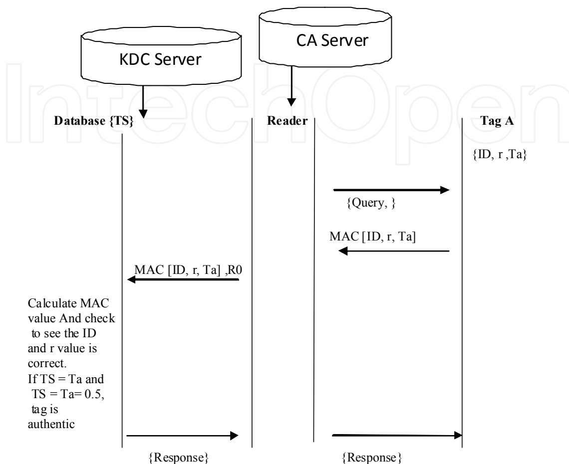
Fig. 4. Cloning Prevention Method
