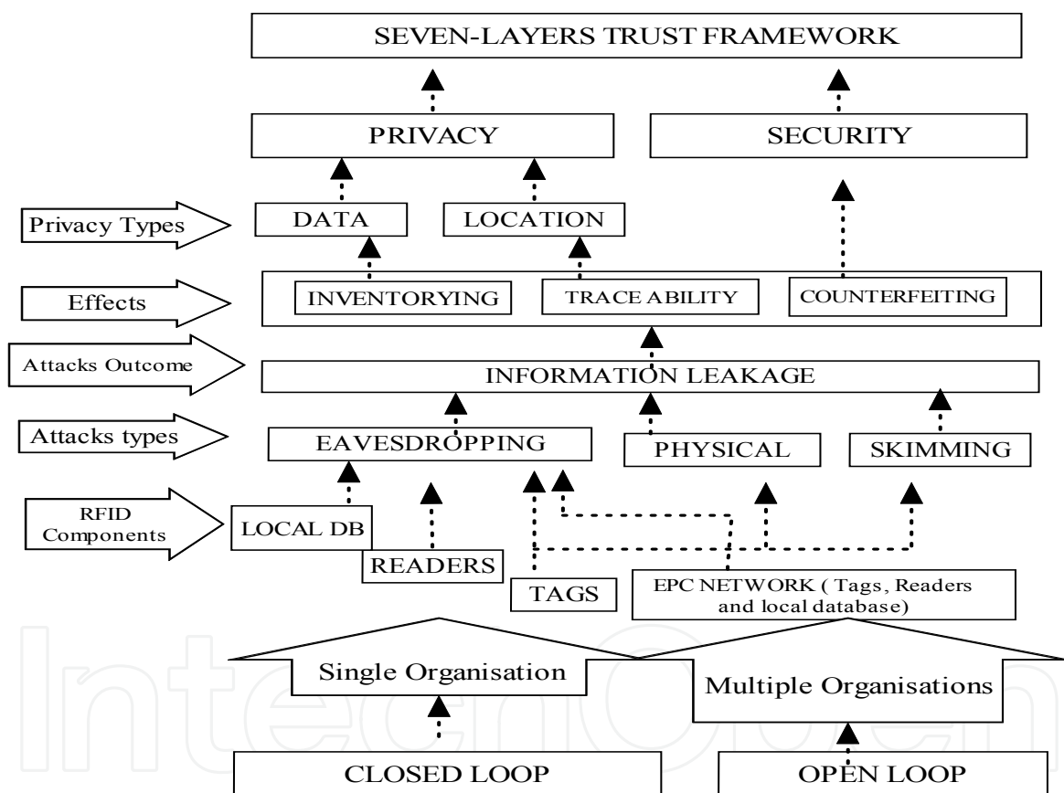
Fig. 2. RFID Privacy Concerns Categorisation
