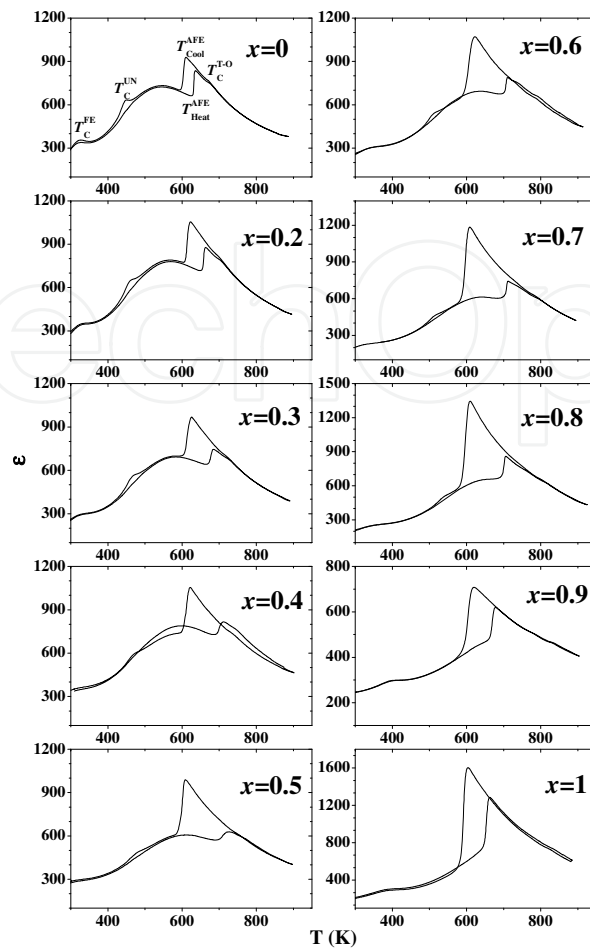
Fig. 16. Temperature dependence of dielectric constants for \text{Ag}_{1-x}\text{Na}_x\text{NbO}_3 solid solutions.
