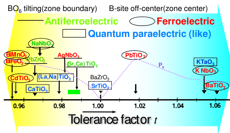
Fig. 2. Tolerance factor of typical dielectric oxides.
