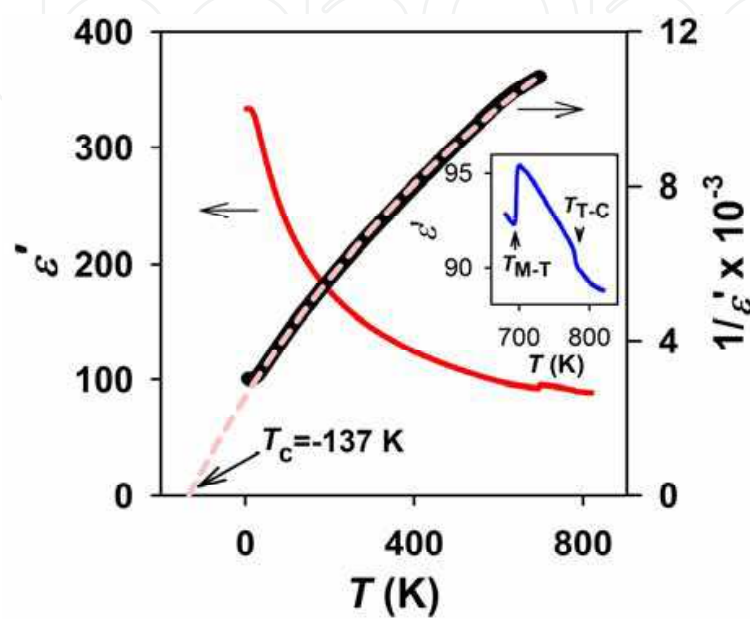
Fig. 26. Temperature dependences of \epsilon' and 1/\epsilon' fitted to the modified Curie-Weiss law \epsilon = \epsilon_L + C/(T - T_0) (dashed line, \epsilon_L = 38.2 , C = 4.7 \times 10^4 K, T_0 = -137 K) for \text{AgTaO}_3 measured at 1 MHz upon heating. The inset further shows the step-like phase transitions from monoclinic to tetragonal and then to cubic at T_{M-T} = 694 K and T_{T-C} = 780 K, respectively.
