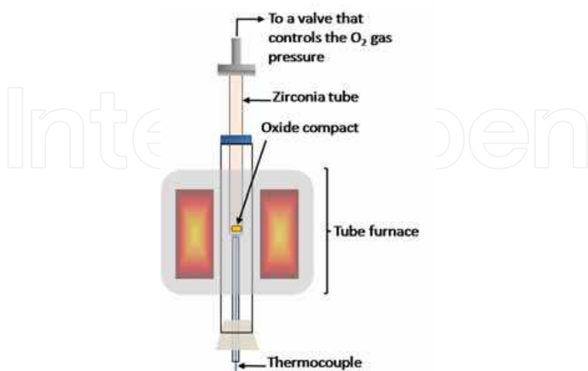
Fig. 22. Schematic diagram of the self-customized furnace employed for the sintering at high oxygen pressure.
