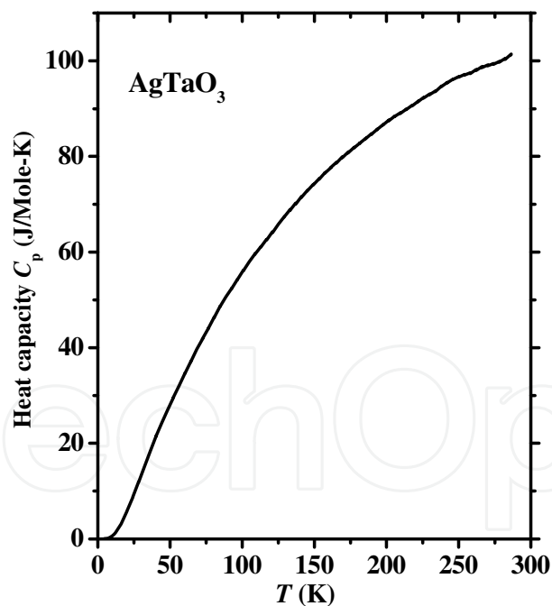
Fig. 25. Heat capacity for \text{AgTaO}_3 .
