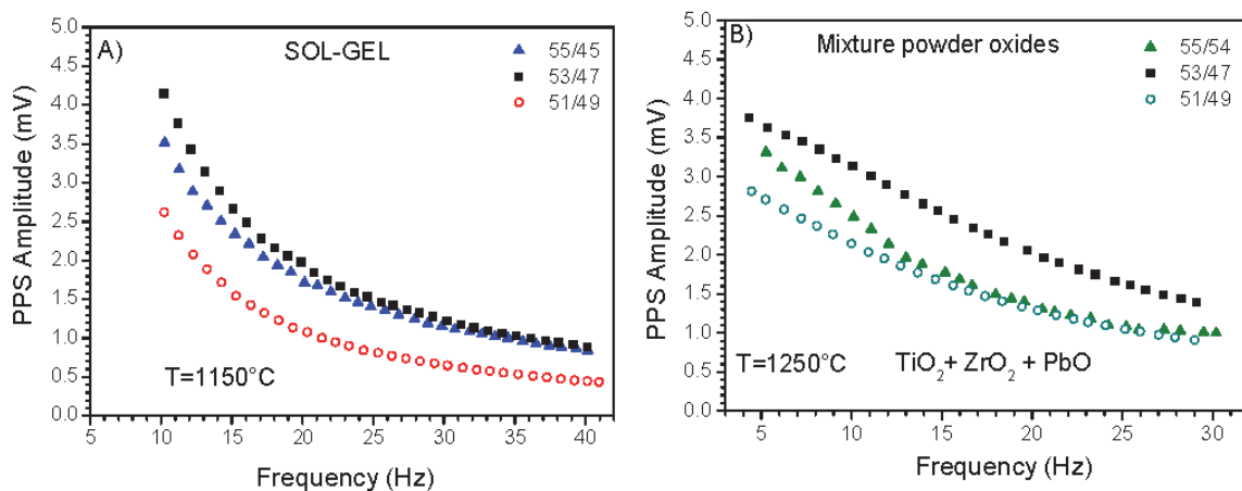
Fig. 9. Pyroelectric response in PZT samples with compositions 55/45, 53/47 and 51/49 obtained by A) Sol-gel method and B) mixture oxides with mechanical activation using PbO as Pb source
