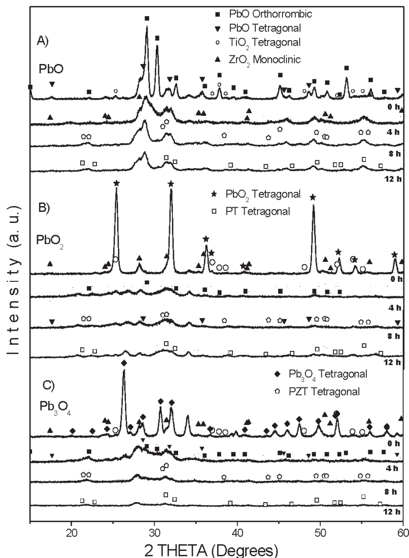
Fig. 1. Evolution of the XRD patterns with milling time of the mixture starting oxides, of three studied set of samples, A) (ZrO 2 , TiO 2 , PbO), B) (ZrO 2 , TiO 2 , PbO 2 ) and C) (ZrO 2 , TiO 2 , Pb 3 O 4 )
