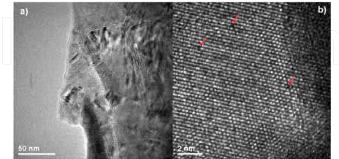
Fig. 9. TEM images of KNN sintered at 1080°C, a) BF and b) HR.
