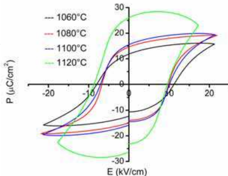
Fig. 8. Ferroelectric loops of KNN ceramics.
