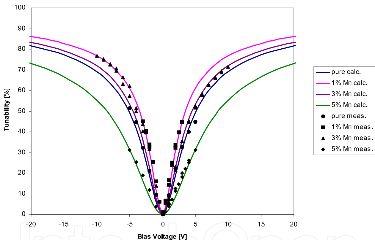
Fig. 6. Comparison of the measured and calculated tunability of (\text{Pb}_{0.4}, \text{Sr}_{0.6})(\text{Ti}_{1-x}, \text{Mn}_x)\text{O}_3 . The fitting parameters C_{\max}[\text{nF}]/V_2[\text{V}] are: pure 9.5/5.1; 1% 15/3.5; 3% 13.8/4.5; 5% 5.7/8.5
